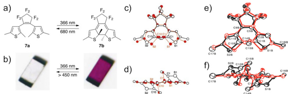
Figure 4. (a) Molecular structure of diarylethene 7 that is photochromic in the single crystal. (b) Photograph of a single crystal of 7a under polarized light before (left) and after (right) UV irradiation. (c) Top view and (d) side view of the movement of each atom of 7a in the crystal during photoisomerization and relative atom positions of 7a (O, open circles) and 7b (b, red circles). (e) Top view and (f) side view of the molecular structure of a crystal of 1b before and after irradiation with 680 nm light for 100 h: The closed-ring form 1b and open-ring form 1a resulting from irradiation were drawn by red and black lines, respectively. The ellipsoids are drawn at the 50% probability level. Hydrogen atoms were omitted for clarity. (Adapted with permission from references 16 and 17. Copyright 1999 and 2000 American Chemical Society).
