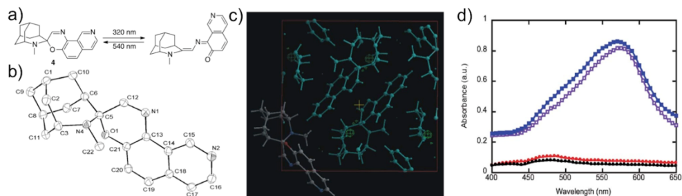
Figure 3. (a) Molecular structure and photoisomerization of SO 4 , (b) crystal structure of SO 4 , (c) the electron density difference map of a single crystal of 4 before and after irradiation with UV light, and (d) polarized absorption spectra of 4 before UV irradiation with the polarizer at 0° (red circles) and 90° (black circles), and after irradiation with the polarizer at 0° (purple squares) and 90° (blue squares) relative to the [011] plane. The electron density difference map is defined as the difference between the electron density map of an irradiated single crystal and that of the same crystal before irradiation. Thermal ellipsoids are shown at the 50% probability level with hydrogens omitted for clarity. (Figure adapted from reference 13. Reproduced by permission of The Royal Society of Chemistry).
