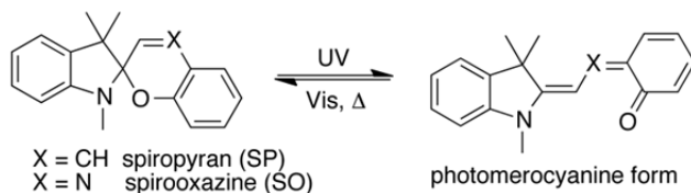
Scheme 1. General structure of spiropyran and spirooxazine. Photoisomerization is initiated with UV light; visible light or heat affects the ring closing reaction.
