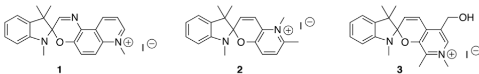
Figure 2. Molecular structures of cationic spiropyran and spirooxazines that show photochromism in microcrystalline powders.
