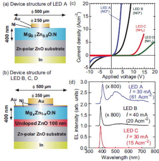
Figure 16. a) and (b) depict cross-sectional schematics for LED A and those of B-D, respectively. The device was 500 \mu m in diameter and the back side of the ZnO substrates was bonded to a metal plate with In. The top electrode in (a) was formed as Au(200nm)/Ni(10nm) with a diameter of 250 \mu m. That of (b) consists of a semitransparent electrode of Au (4nm)/Ni (2nm) with a diameter of 500 \mu m and a contact pad of Au (500nm)/Ni (2nm) with a diameter of 350 \mu m. (c) The rectifying I - V curve measured for LEDs A, B, C, and D. (d) EL spectra from LEDs A-C. All spectra were measured at room temperature. Forward bias operation conditions are also shown. From Ref. [81].
