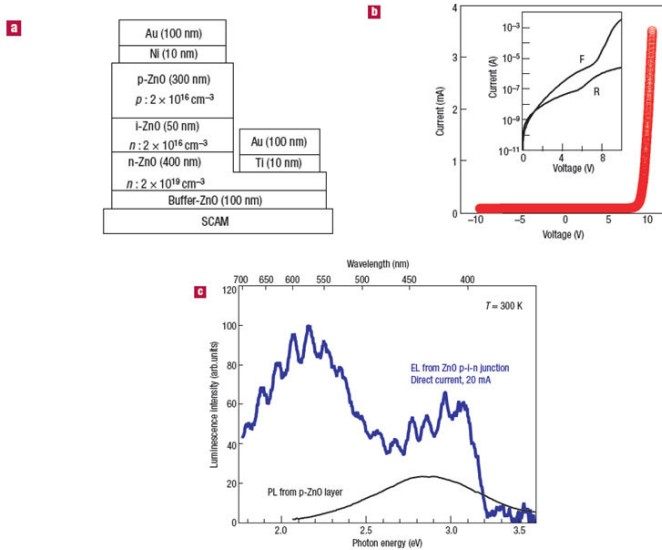
Figure 1. ZnO homostructural p-i-n junction shows rectifying current-voltage characteristics and electroluminescence (EL) in forward bias at room-temperature. (a), The structure of a typical p-i-n junction LED. (b), Current-voltage characteristics of a p-i-n junction. The inset has logarithmic scale in current with F and R denoting forward and reverse bias conditions, respectively. (c), Electroluminescence spectrum from the p-i-n junction (blue) and photoluminescence (PL) spectrum of a p-type ZnO film measured at 300 K. The p-i-n junction was operated by feeding in a direct current of 20 mA. From Ref.[5].
