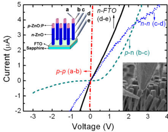
Figure 22. I-V characteristics of p-p , p-n , n-n , and n-FTO regions in a single ZnO rod. The upper left and lower right insets show the schematic diagram and a SEM image of probing by Zyvex nanomanipulator, respectively. From Ref. [97].
