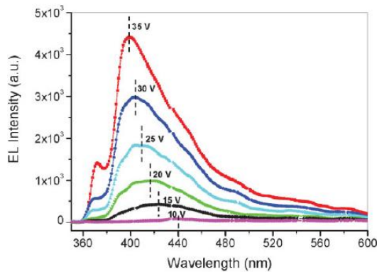
Figure 9. The electroluminescence spectrum of the (n-ZnO NWs)/(p-GaN film) LED device under various forward bias voltages (10, 15, 20, 25, 30, 35V), showing broad emission peaks from UV to blue and blue shift with increasing of bias voltage. From Ref. [69].
