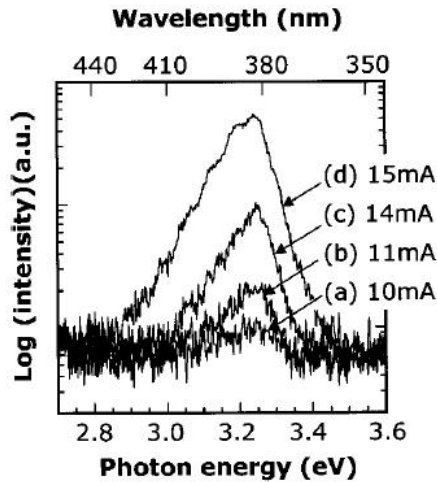
Figure 7. UV emission spectra of the p\text{-SrCu}_2\text{O}_2/n\text{-ZnO} p-n junction LED for several currents. electric currents were (a) 10mA, (b) 11mA, (c) 14mA, and (d) 15mA, respectively. From Ref. [56].
