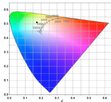
Figure 12. Typical color coordinates characteristics of the ZnO – PFO hybrid white LEDs. From Ref. [65].
