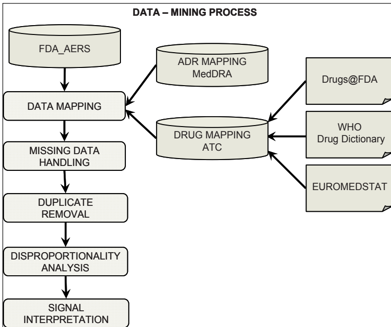
Figure 5. Steps of FDA_AERS data-mining process
