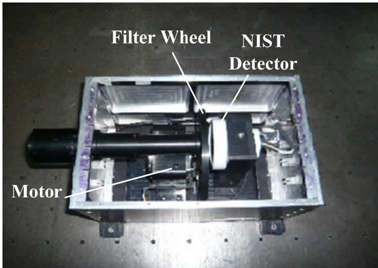
Figure 6. The structure of the HAUVSR
