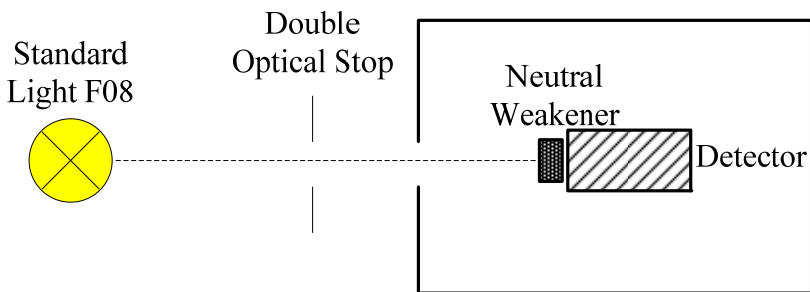
Figure 9. Detector Linearity testing facility
