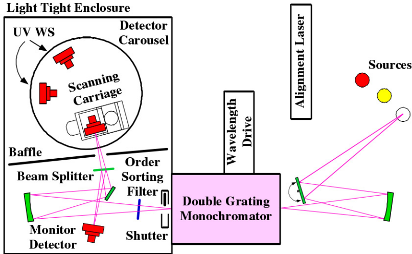
Figure 5. Ultraviolet Spectral Comparator Facility (UV SCF)
