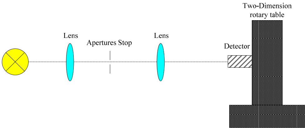
Figure 7. Detector Space Uniformity testing system
