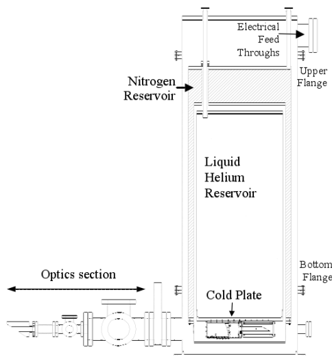
Figure 1. The construction of the NIST Primary Optical Watt Radiometer(POWER)
