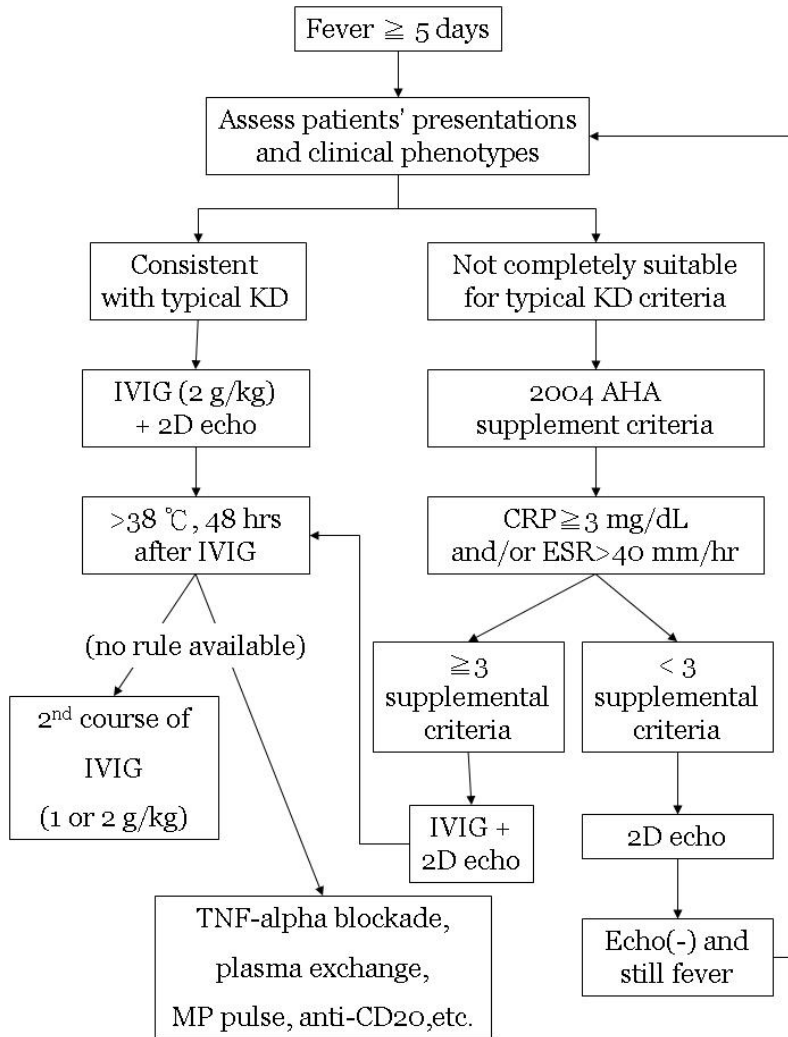
Figure 9. Flowchart of Kawasaki disease management
