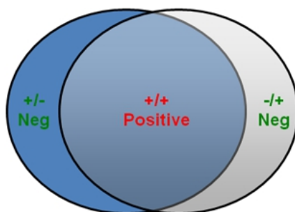
Fig. 8. Diagram representing a duplex real-time PCR assay for detection of Salmonella Typhimurium. Each assay detects S. Typhimurium plus some non-Typhimurium strains. Because each assay detects a different set of non-Typhimurium strains, only when both assays are positive is the sample positive for S. Typhimurium . The assays are labeled with a different fluorophore to be detected independently by real-time PCR.
