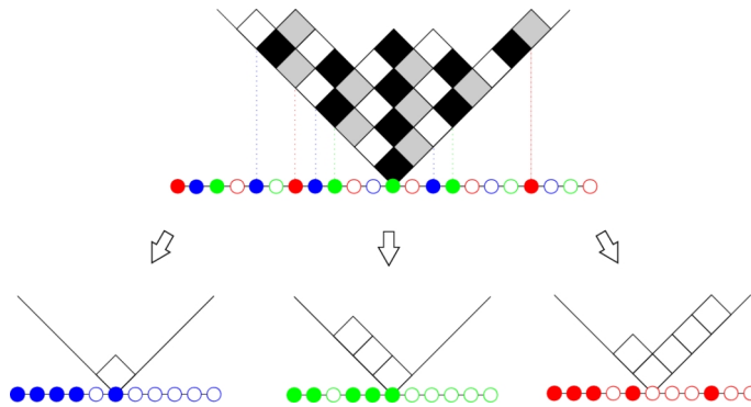
Figure 5. The decomposition of the partition for \mathbb{Z} r=3 . First suppose the standard correspondence between the one-dimensional particles and the original partition, and then rearrange them with respect to mod r .
