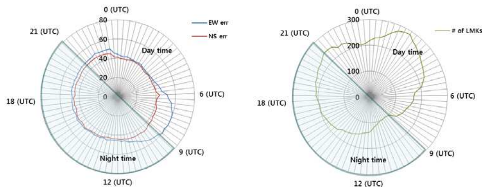
Fig. 23. MI INR performance during 1 st April ~ 31 th August.
