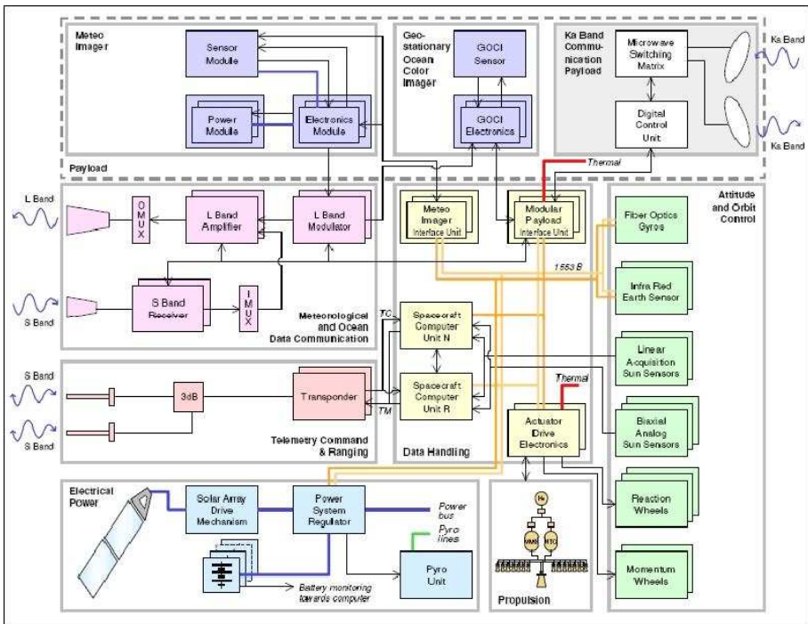
Fig. 3. Block diagram of COMS spacecraft functional architecture
