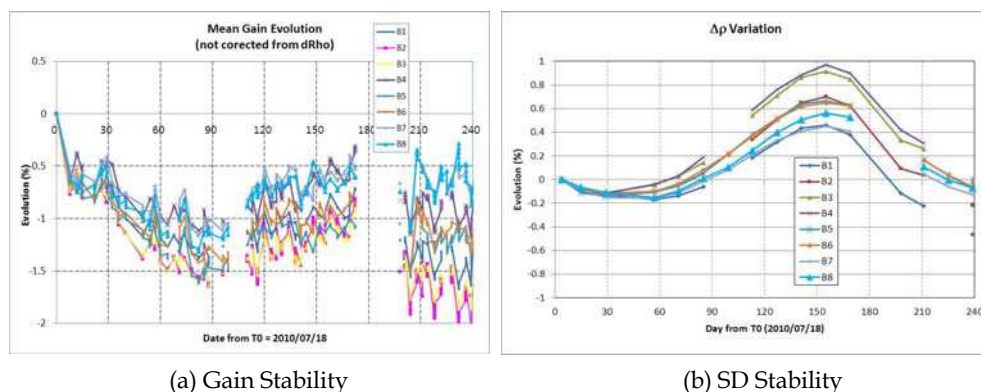
Fig. 20. In-orbit radiometric stability over 8 months
