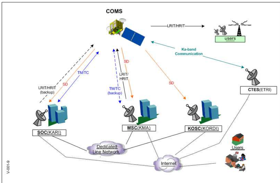
Fig. 2. COMS system overview
