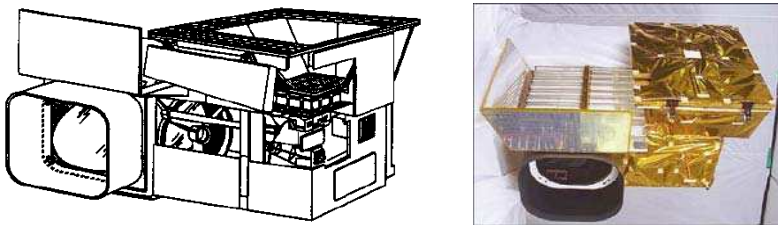
Fig. 4. COMS MI sensor module, in design and flight model configurations
