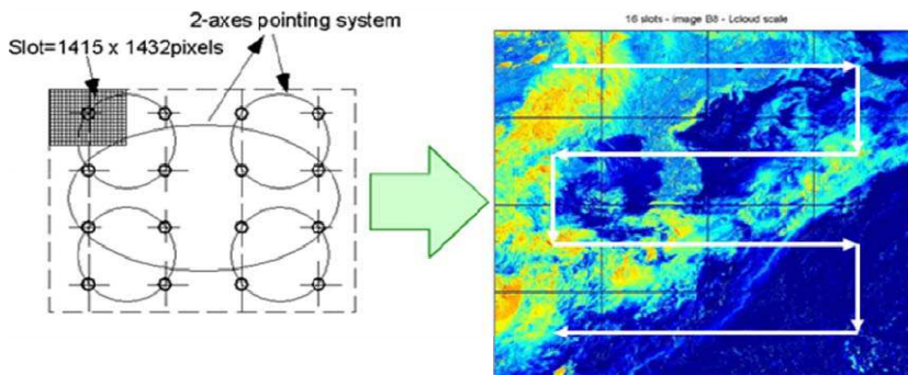
Fig. 10. GOCI imaging principle
