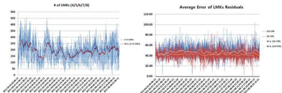
Fig. 23. MI INR performance during 1 st April ~ 31 th August.
