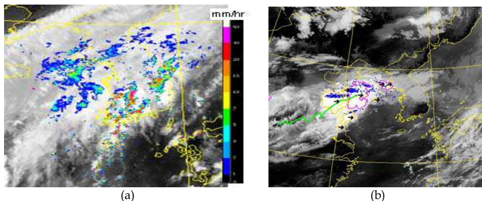
Fig. 27. Examples of COMS MI data applications (a) Convective rain intensity image combined with radar rain map (b) Predicted location of convective cloud and lightning image.
