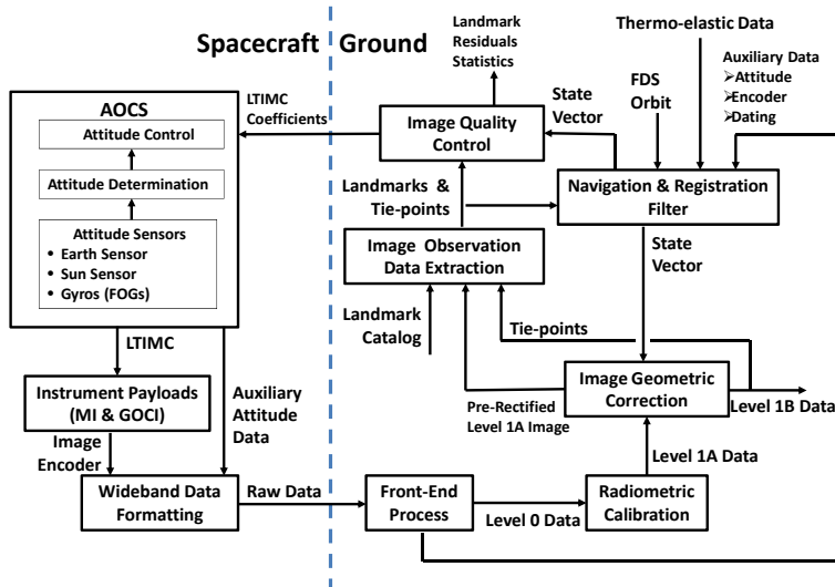
Fig. 11. COMS INR overall architecture
