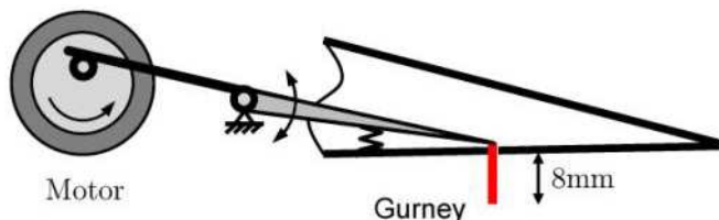
Fig. 11. Mini-flap Gurney type electromechanical movement (schematic).
