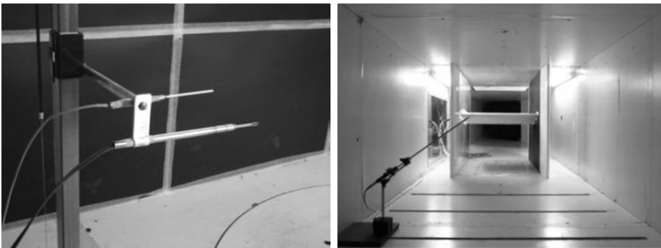
Fig. 9. Experimental setup views.
