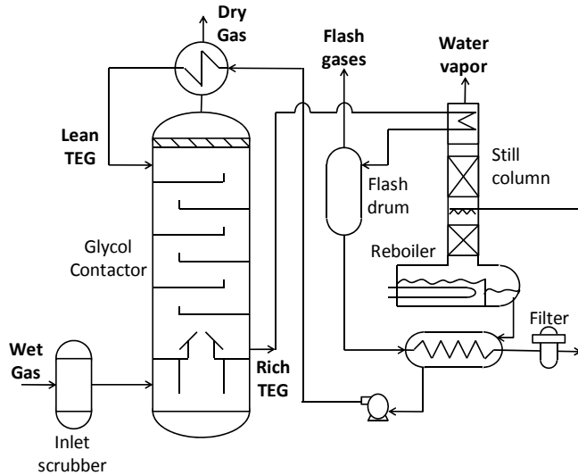
Figure 2. TEG absorption dehydration scheme
