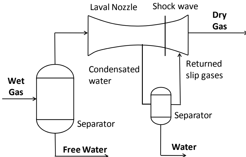
Figure 10. Scheme of a supersonic dehydration line
