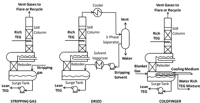
Figure 3. Enhanced TEG regeneration systems
