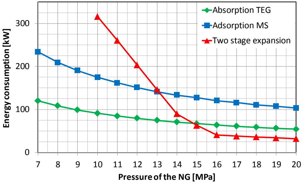
Figure 13. Energy consumption results for conventional dehydration methods
