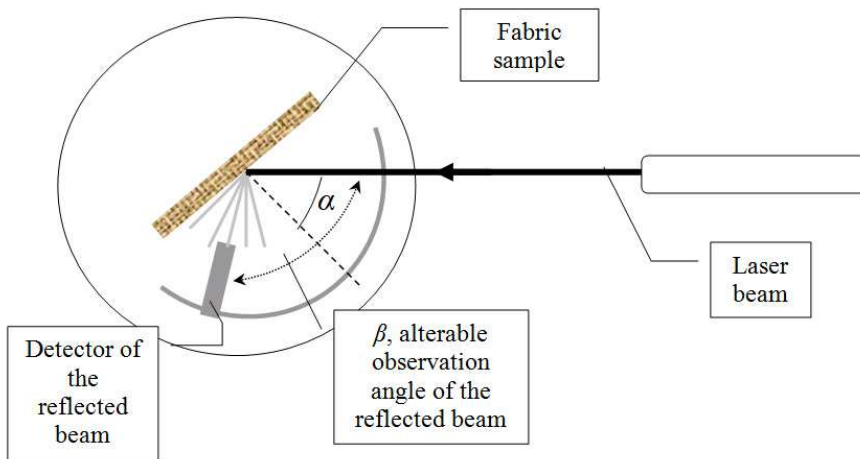
Fig. 6. Scheme of the reflection study experiment
