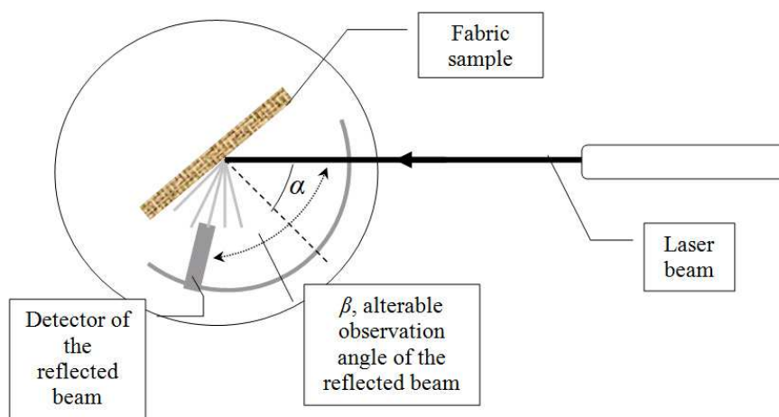
Fig. 6. Scheme of the reflection study experiment
