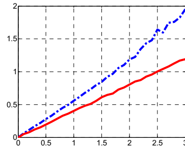
Figure 7. The reprojection error versus \sigma . The dashed line represents the results obtained by using the linear minimization alone. The solid line shows the results after the non linear refinement. Both units are considered in pixels
