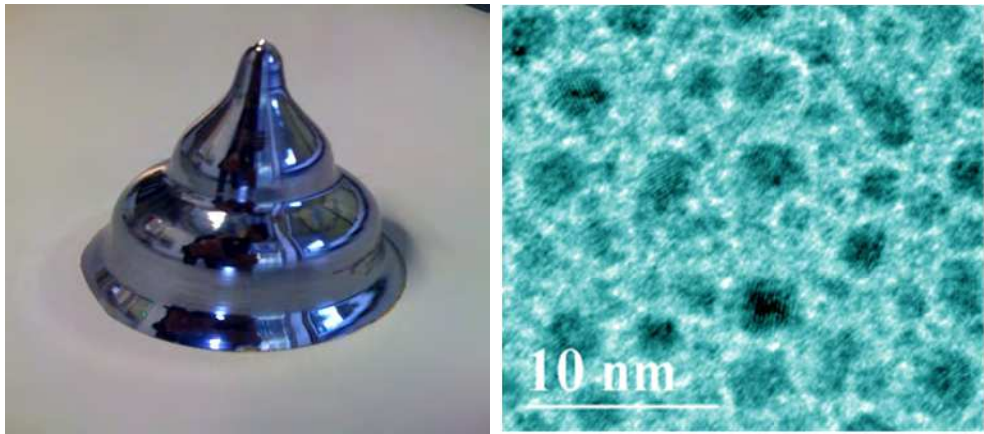
Fig. 3. (left) Upper part of an ingot of single crystalline silicon. The diameter of the ingot shown in the photograph is 100 mm. Largest silicon ingots grown by the Czochralski method have a diameter of 30 mm and a length of ~2m. (right) HRTEM image of tiny silicon quantum dots in a SiO 2 matrix. Si-dots appear as dark structures and the (111) lattice plans are clearly seen. The dimension of the Si-quantum dots shown in the image is between 2 and 5 nm.
