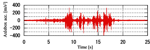
(a) Vertical acceleration of axle-box
