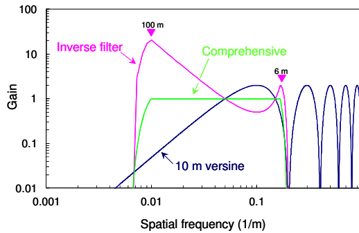
Fig. 31. Inverse filter for track profile restoration
