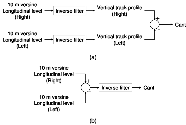
Fig. 30. Calculation flow for cant
