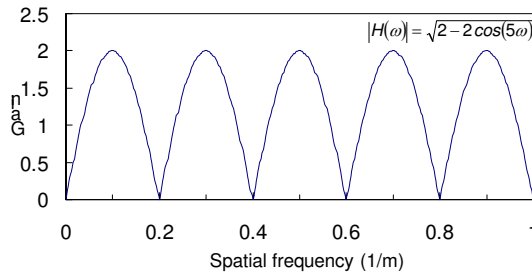
Fig. 27. Frequency response of difference filter
