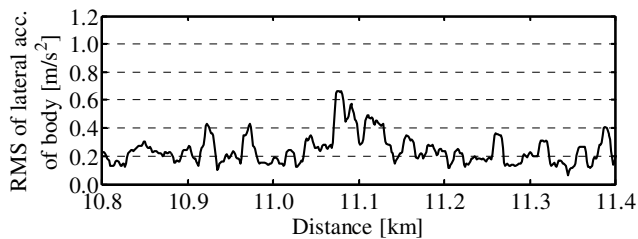
(b) RMS of lateral acceleration of car body
