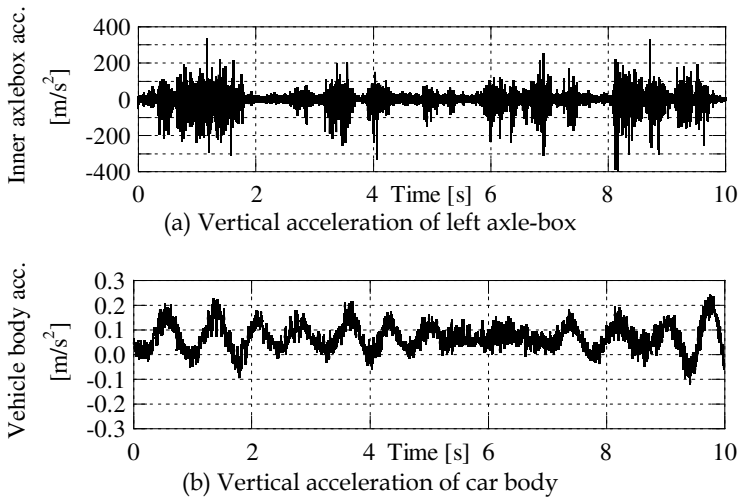
Fig. 3. Measurement results of curved section with corrugation
