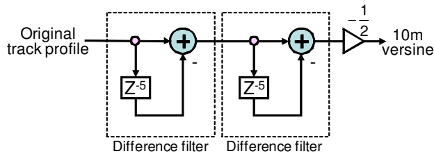
Fig. 26. Brock diagram of 10 m versine method
