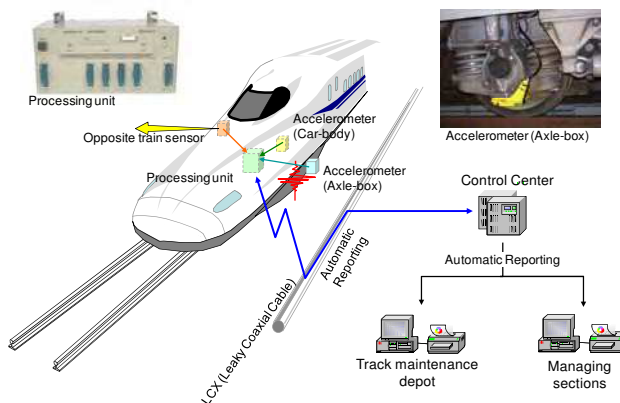
Fig. 23. RAIDARSS-3: Track condition monitoring system for Tokaido shinkansen
