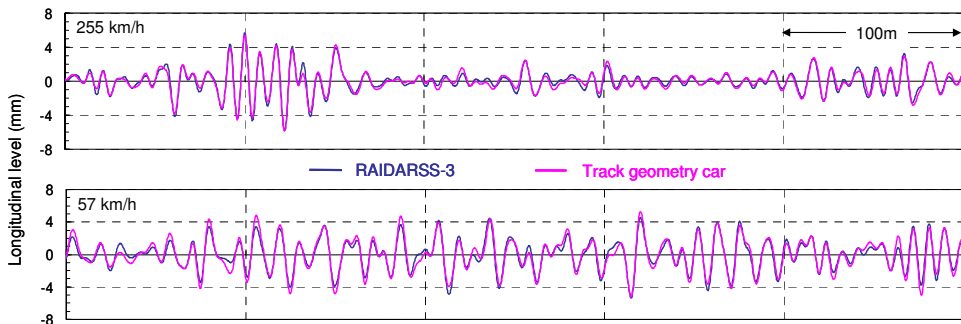
Fig. 29. Comparison between RAIDARSS-3 and Dr. Yellow
