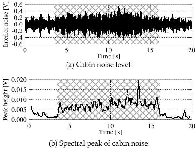
Fig. 12. Cabin noise measured at in-service vehicle and its spectral peak
