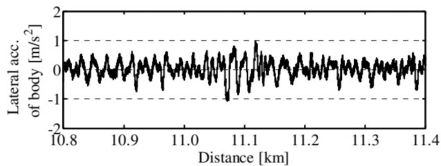
(a) Lateral acceleration of car body
