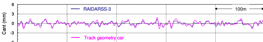
Fig. 32. Cant calculated from RAIDARSS-3
