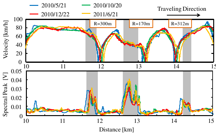
Fig. 21. Spectral peak of cabin noise
