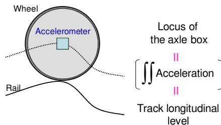
Fig. 24. Inertial track measurement in longitudinal level
