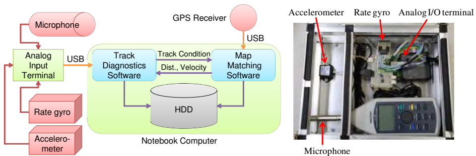
Fig. 13. Portable onboard sensing system
