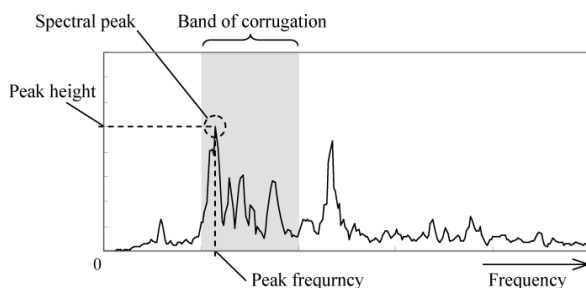
Fig. 11. Detection of corrugation from cabin noise
