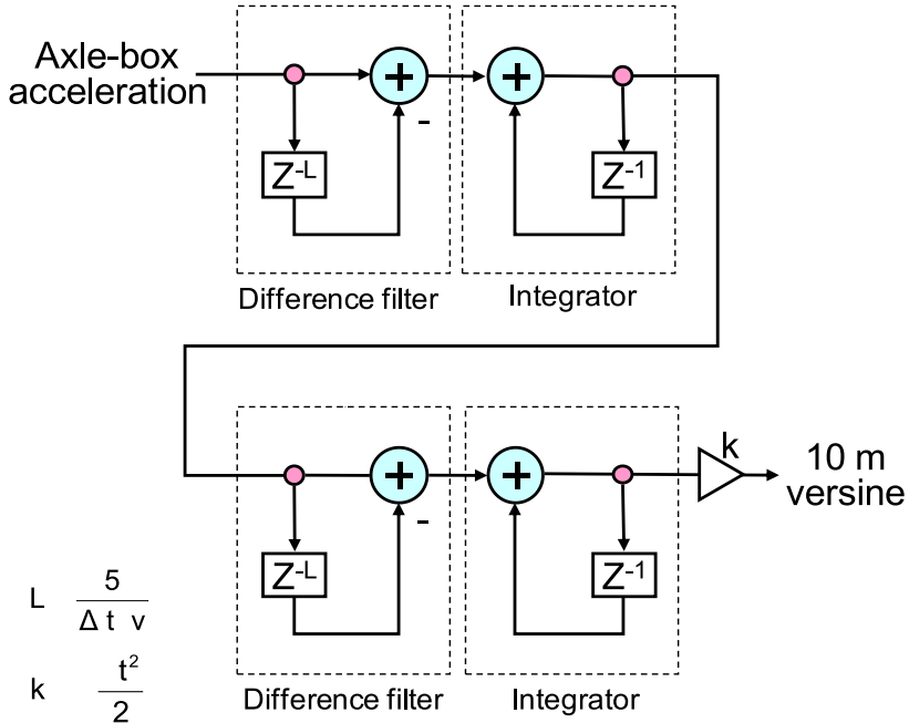
Fig. 28. Block diagram of frequency variable difference filter
