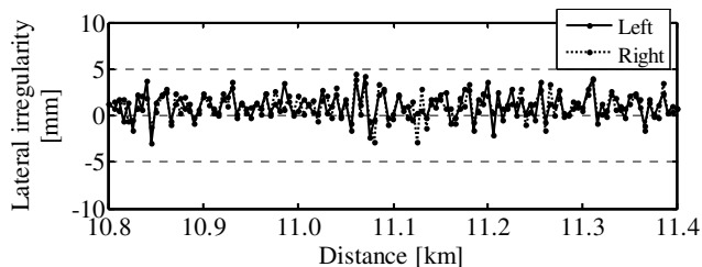
(c) Lateral irregularity of track
