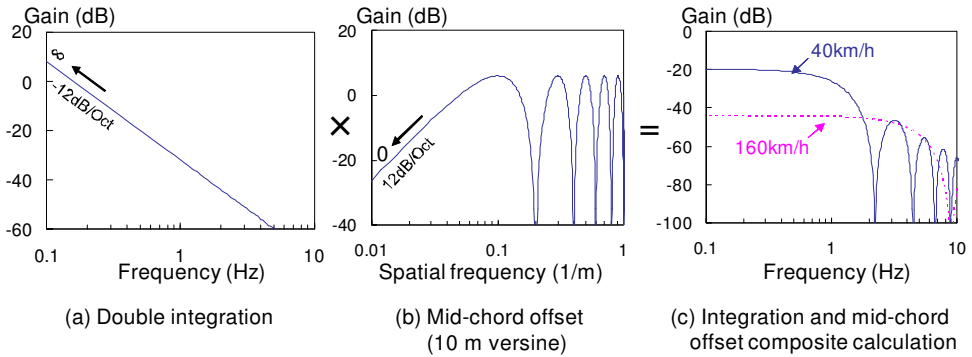
Fig. 25. Digital inertial processing for RAIDARSS-3
