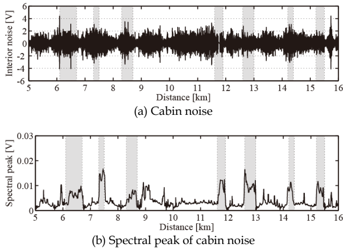
Fig. 18. Detection of corrugation
