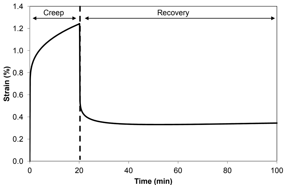
Fig. 6. The creep and recovery curve of SBS
