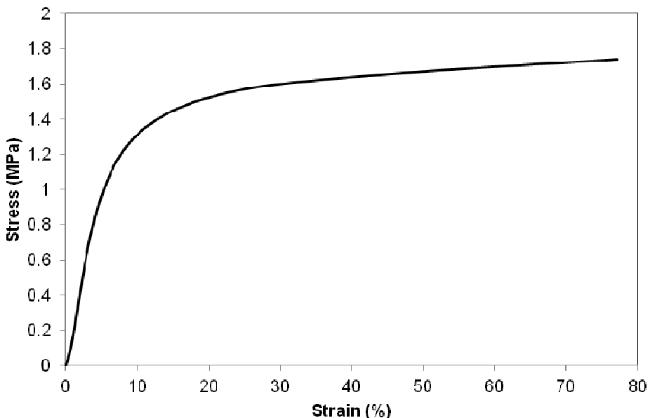
Fig. 4. The stress-strain curve of SBS
