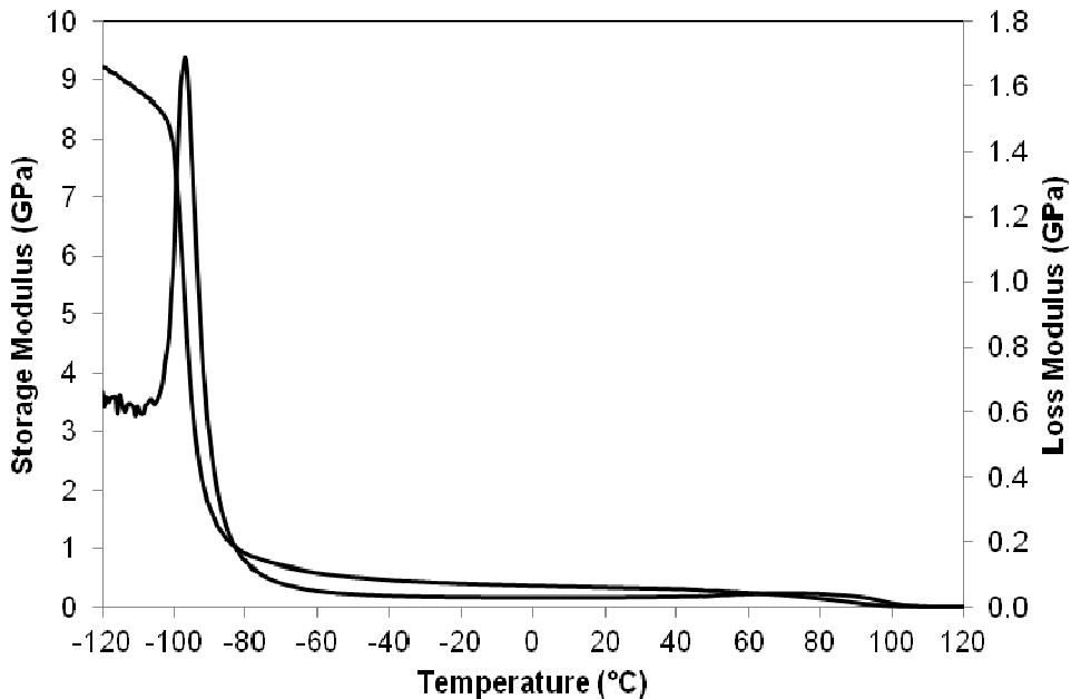
Fig. 5. The storage and loss modulus curves of SBS
