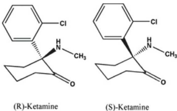
Fig. 2. Chemical Structure of Ketamine
