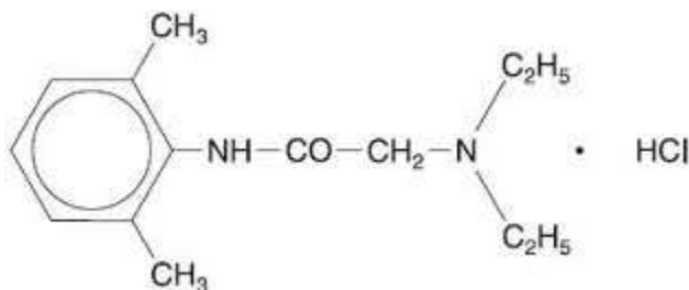
Fig. 3. Lidocaine chemical structure
