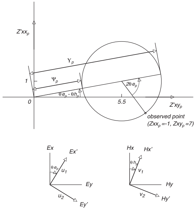
Fig. 6. Diagram showing the Mohr representation and the SVD of the matrix in Equation 37. The values of \theta e_p , \theta h_p , Y_p and \Psi_p are evident as 32^\circ , 21^\circ , 8.1 and 3.1 . The axes for E'_x , E'_y and H'_x , H'_y show the rotations, from E_x , E_y and H_x , H_y by \theta e_p and \theta h_p respectively, to give an ideal 2D antidiagonal response.
