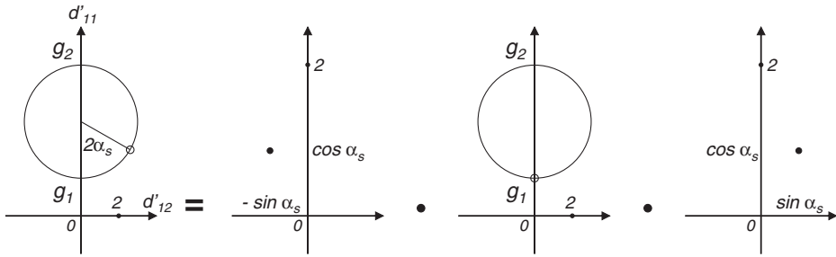
Fig. 10. Mohr diagrams for the decomposition in Equation 54. On the left the diagram shows the distortion matrix \mathbf{d} . It is positive definite, due to the assumption of strictly 2D surficial anisotropy, and so has orthogonal eigenvectors. The radius of the circle is (g_2 - g_1)/2 . The numerical matrix taken for the example is [3.5, 2.6; 2.6, 6.5] , and the directions and magnitudes of its eigenvectors are shown by rotating the radial arm until it is parallel to the vertical axis. The eigenvalues then are g_1 = 2 and g_2 = 8 . The angle 2\alpha_s on the figure is 60^\circ , indicating that a rotation of axes anticlockwise through 30^\circ is necessary to change the matrix to [2, 0; 0, 8] . On the right is shown the matrix decomposition as in Equation 54. The three diagrams represent the three matrices on the right-hand side of that equation, in turn. The first Mohr diagram represents a rotation by angle (-\alpha_s) . The second Mohr diagram is symmetric, representing a positive definite matrix according to the scaling factors g_1 and g_2 . The third matrix is like the first, representing a rotation by angle (+\alpha_s) . Note the changes of scale between the diagrams.
