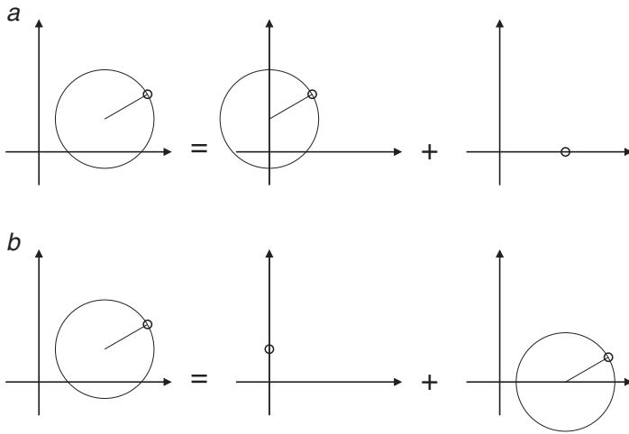
Fig. 4. Separation of a 2 x 2 matrix, a: into symmetric and 1D parts as in Equation 18; b: into symmetric and 2D parts as in Equation 20. The diagrams are drawn for Z = [1.75, 3.30; -0.70, 0.25] . Thus case a is: Z = [1.75, 1.3; 1.3, 0.25] + [0, 2.0; -2.0, 0] , and case b is: Z = [1.0, 0; 0, 1.0] + [0.75, 3.3; -0.7, -0.75] .
