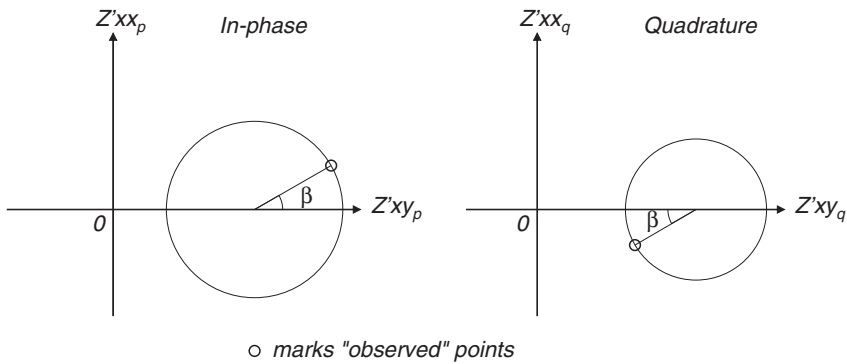
Fig. 11. Hypothetical example of a 2D case with the in-phase and quadrature radial arms anti-parallel. Such cases appear to be prohibited in nature, but inadvertently can be posed as numerical examples.
