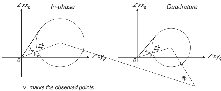
Fig. 3. Seven invariants of rotation for a general 3D MT tensor.
