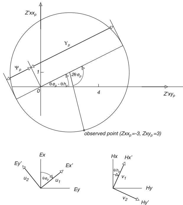
Fig. 12. The Mohr diagram for the matrix in Equation 70. The circle encloses the origin of axes because the matrix has a negative determinant. The values of \theta_{e_p} , \theta_{h_p} , Y_p and \Psi_p are evident as 51^\circ , 25^\circ , 6.3 and -1.8 ( \Psi_p being of negative sign when the direction of Y_p from the origin defines positive).
