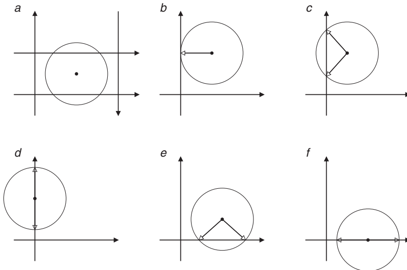
Fig. 5. Eigenvector directions (according to the radial arrows) and eigenvalues (where the arrowheads touch an axis) displayed on Mohr diagrams for a 2 \times 2 matrix. a: Eigenvalues are complex conjugates, and are not evident on the diagram. b: Eigenvalues are real and equal; both eigenvectors are the same. c: Eigenvalues are real and different; eigenvectors are not orthogonal. d: Eigenvalues are real and different; eigenvectors are orthogonal. e: Associated MT eigenvalues are real and different; eigenvectors are not orthogonal. f: Associated MT eigenvalues are real and different; eigenvectors are orthogonal (the 2D case). In Fig. 5a axes are also drawn for Z'_{yx} and Z'_{yy} . Between the Z'_{xx} and Z'_{yy} axes, the product Z'_{xy} \cdot Z'_{yx} < 0 . On the Z'_{xx} and Z'_{yy} axes, Z'_{xy} \cdot Z'_{yx} = 0 . Outside the Z'_{xx} and Z'_{yy} axes, Z'_{xy} \cdot Z'_{yx} > 0 .
