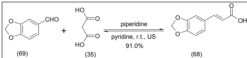
Fig. 21. Ultrasound-catalysed synthesis of Knoevenagel reaction product (68).
