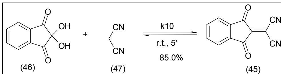
Fig. 12. Knoevenagel product (45) synthesis.
