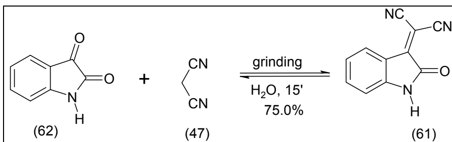
Fig. 19. Isatin compound (61) synthesis.
