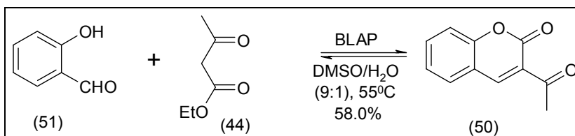
Fig. 14. Coumarin (50) synthesis using BLAP.
