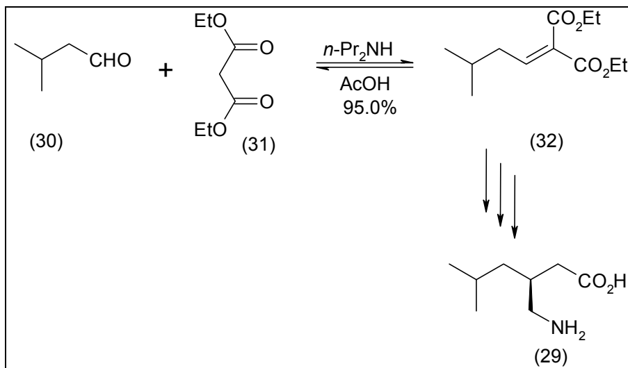
Fig. 7. Pregabalin (29) synthesis.
