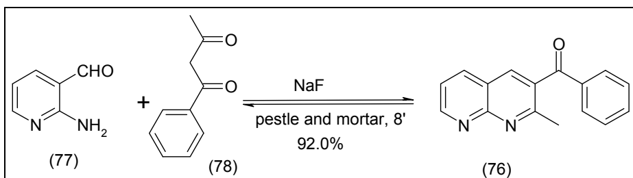
Fig. 24. Synthesis of the Friedlander condensation product (76).
