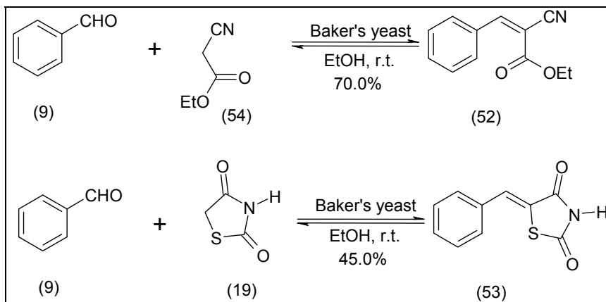
Fig. 15. Knoevenagel reactions using a biotechnology-based approach.
