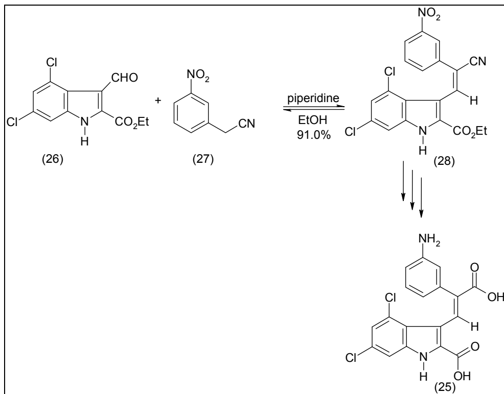
Fig. 6. MDL 103371 (25) synthesis.
