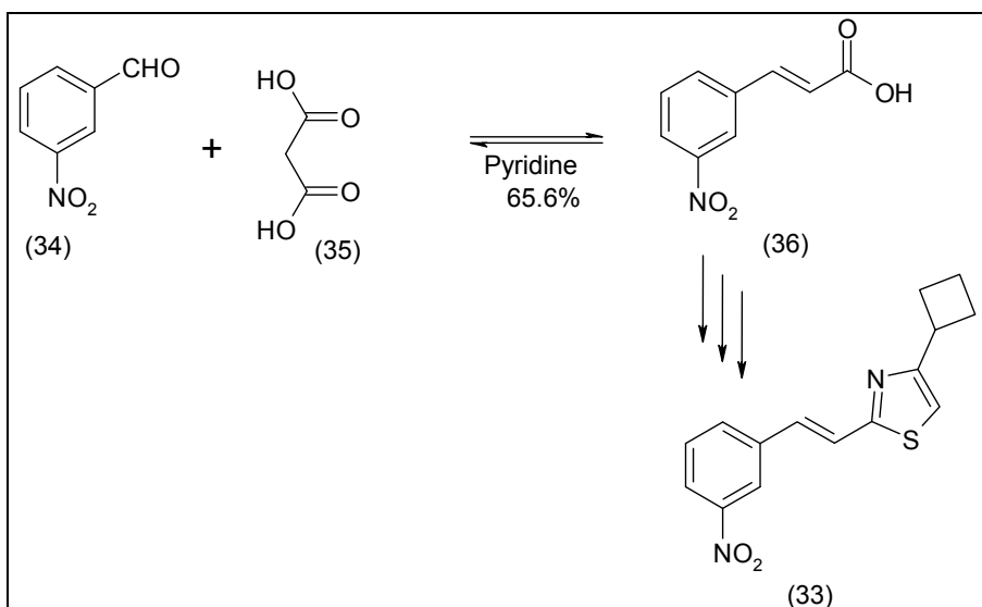
Fig. 8. Ro 24-5913 (33) synthesis.
