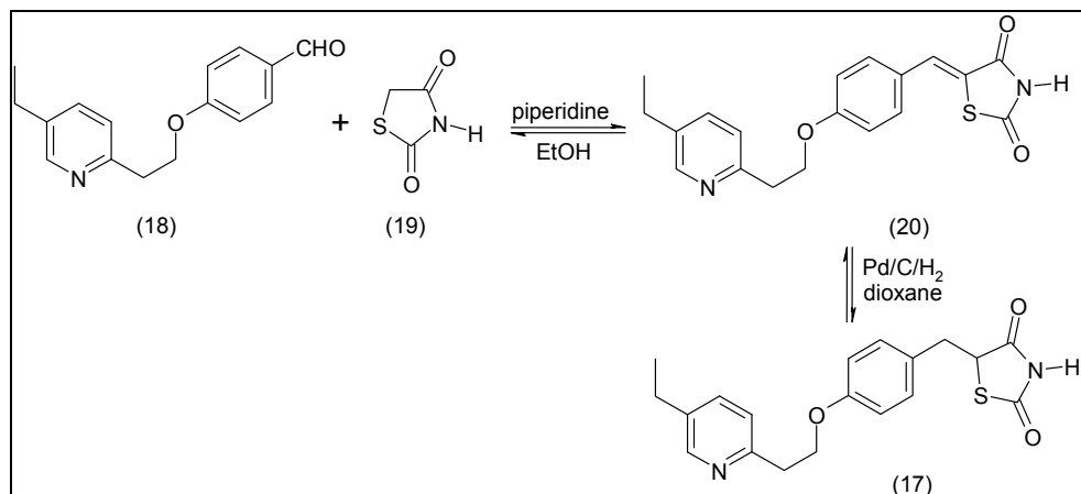
Fig. 4. Selected steps of the pioglitazone (17) synthesis.
