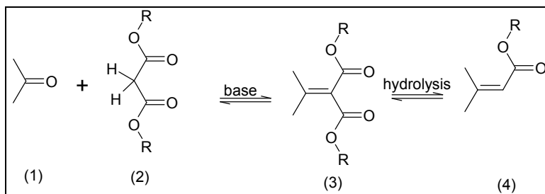
Fig. 1. An example of the Knoevenagel reaction.
