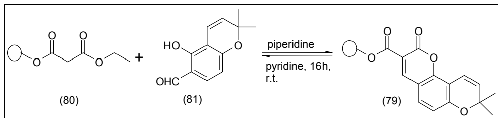
Fig. 25. Synthesis of coumarin (79) via solid phase organic synthesis.
