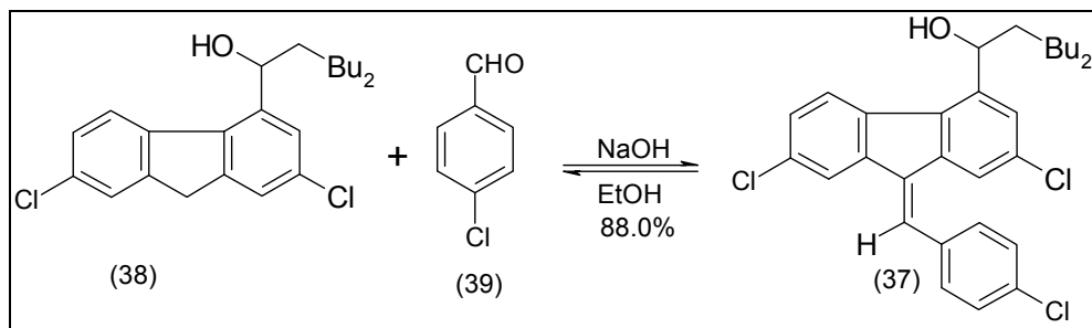
Fig. 9. Lumefantrine (37) synthesis.
