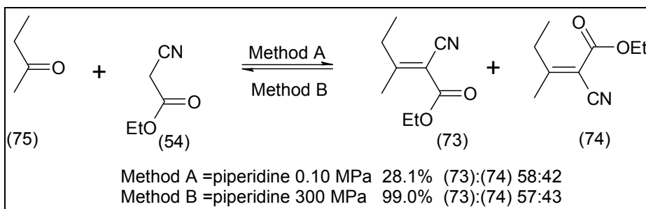
Fig. 23. High-pressure Knoevenagel reactions.
