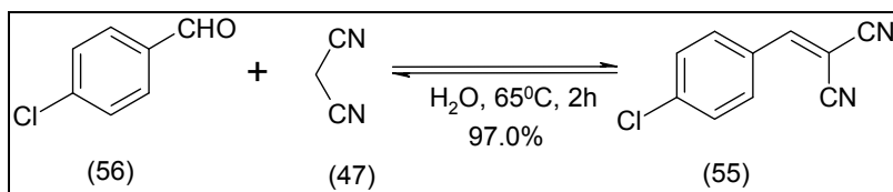
Fig. 16. A Knoevenagel reaction carried out in water.
