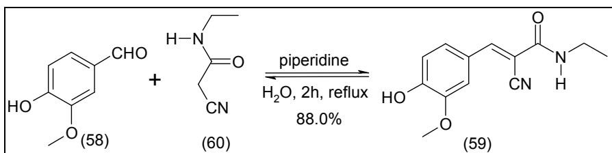
Fig. 18. Compound (59) synthesis.
