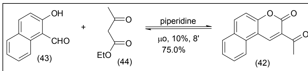
Fig. 11. Coumarinic derivative (42) synthesis.
