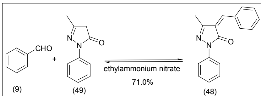
Fig. 13. Compound (48) synthesis.
