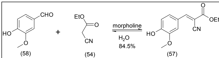
Fig. 17. Morphonile-catalysed synthesis of sunscreen in water.
