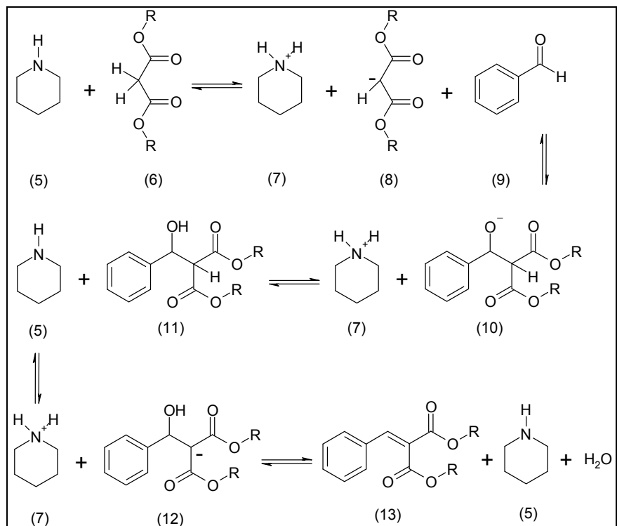
Fig. 2. General mechanism for the Knoevenagel reaction.
