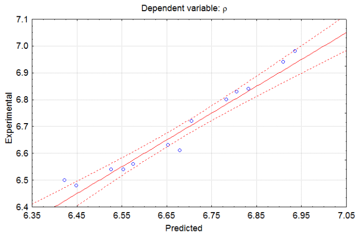
Fig. 14. The dependence between experimental and calculated values of the density.
