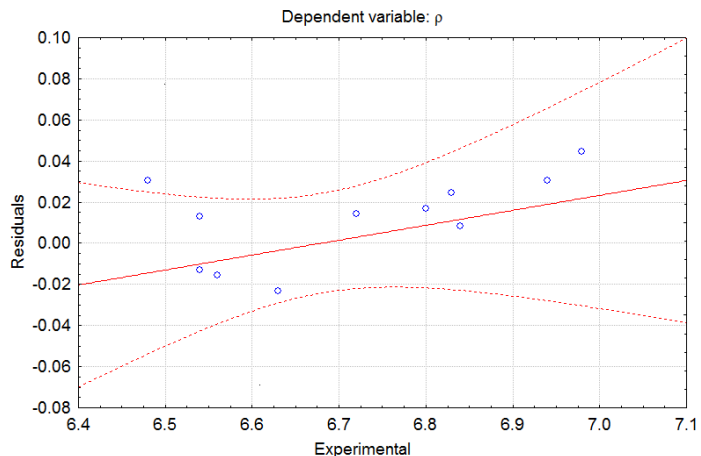
Fig. 15. The dependence between the residuals and experimental values of the density.
