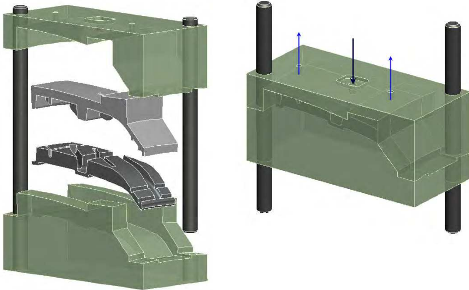
Fig. 11. Die-casting mould.
