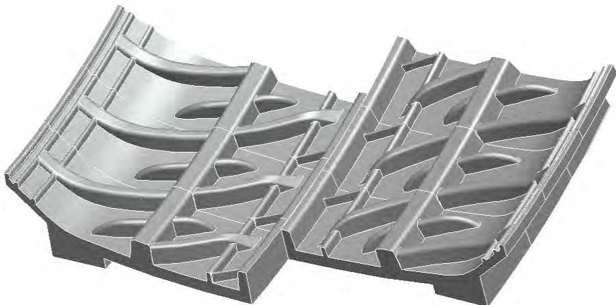
Fig. 14. Assembly of one-pitch-segments makes tread ring (segments).
