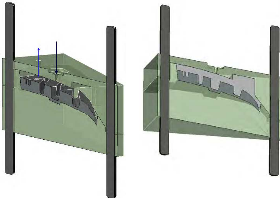
Fig. 12. Die-casting of one-pitch-segment of tread ring.
