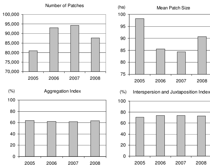
Fig. 6. Spatial characteristics of the phenological cluster aggregates.
