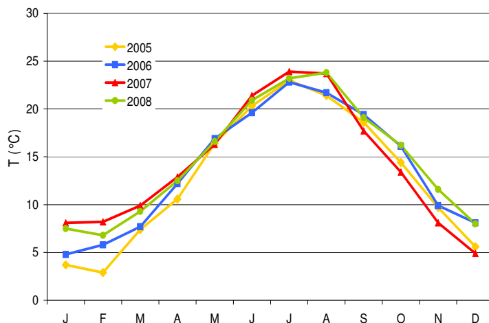
Fig. 9. Mean monthly temperature over the study area.
