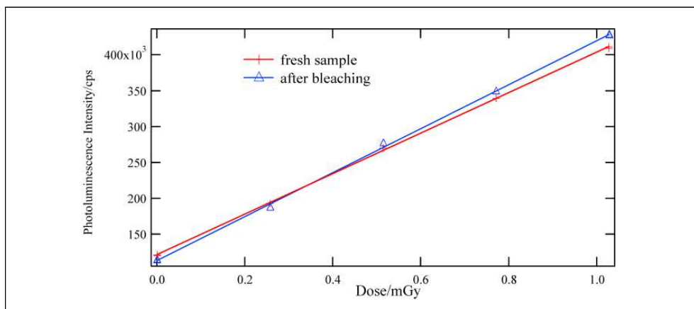
Fig. 12. Reproducibility of nanocrystalline BaFCl:Sm 3+ in dosimetry.
