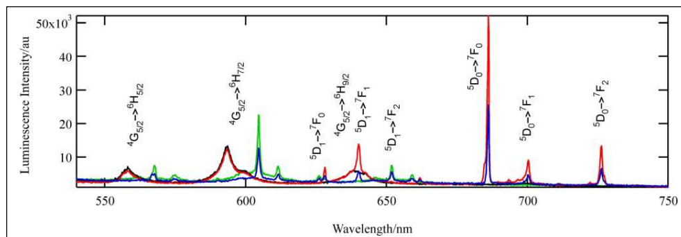
Fig. 10. Photoluminescence of high temperature (green and blue lines) and nanocrystalline (black and red lines) BaFCl:Sm 3+ before and after exposure to 12000 Gy and 50 mGy, respectively. Prominent {}^4G_5 \rightarrow {}^6H_5 (Sm 3+ ) and {}^5D_1 \rightarrow {}^7F_1 (Sm 2+ ) transitions are denoted. Note that the unexposed samples (green and black lines for HT and nano sample, respectively) do not exhibit any emission lines due to Sm 2+ .
