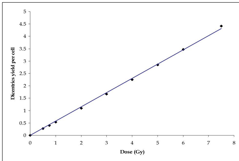
Fig. 4. Dose-effect relationship fitted by scoring of dicentric induced in peripheral blood lymphocytes after in vitro irradiation with fission neutrons (1 MeV). The equation of the curve is Y=0.5356D+3\times 10^{-16}
