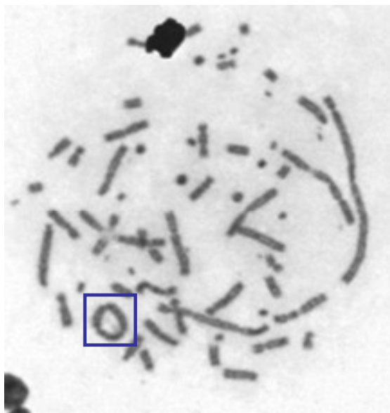
Fig. 5. PCC of peripheral blood lymphocytes in G2. Unstable chromosomal aberrations are analyzed with Giemsa staining. The ring is framed in blue.
