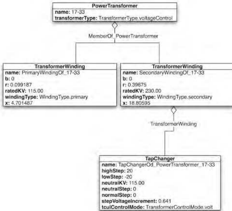
Fig. 9. CIM model of the object Transformer with four sub objects and attributes.
