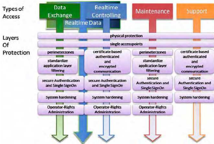
Fig. 15. Defense in depth architectures for different functionalities of Smart grids.
