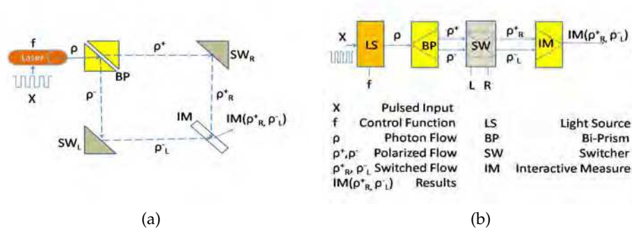
Fig. 1. (a-b) Double Path Model (a) Mach-Zehnder Double Path Model (b) Description Model
