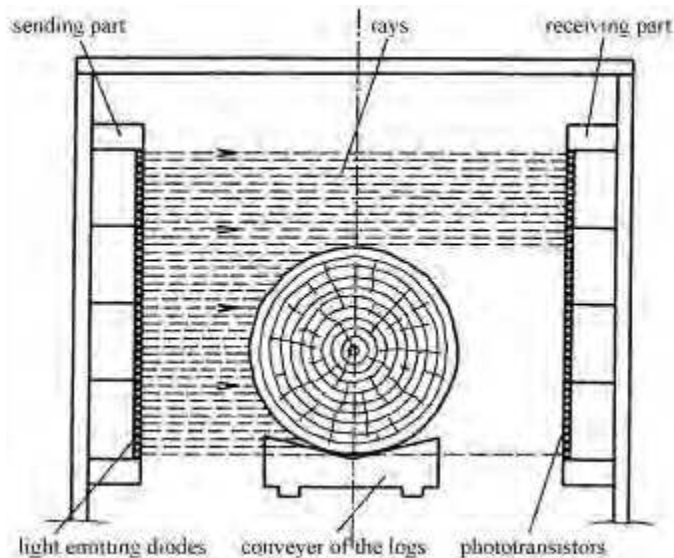
Fig. 3. The principle of scanning the log diameter by a one-directional scanning frame.
