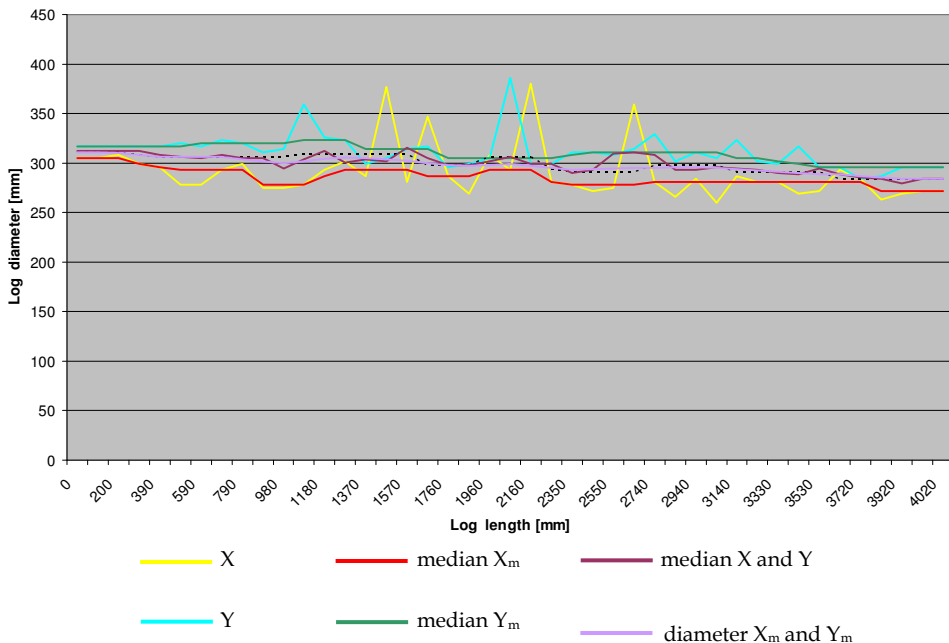
Fig. 8. An example of the effect of various procedures of filtration of scanned data on the resulting image of a log in a control computer (the log shows ragged bark in its central part).
