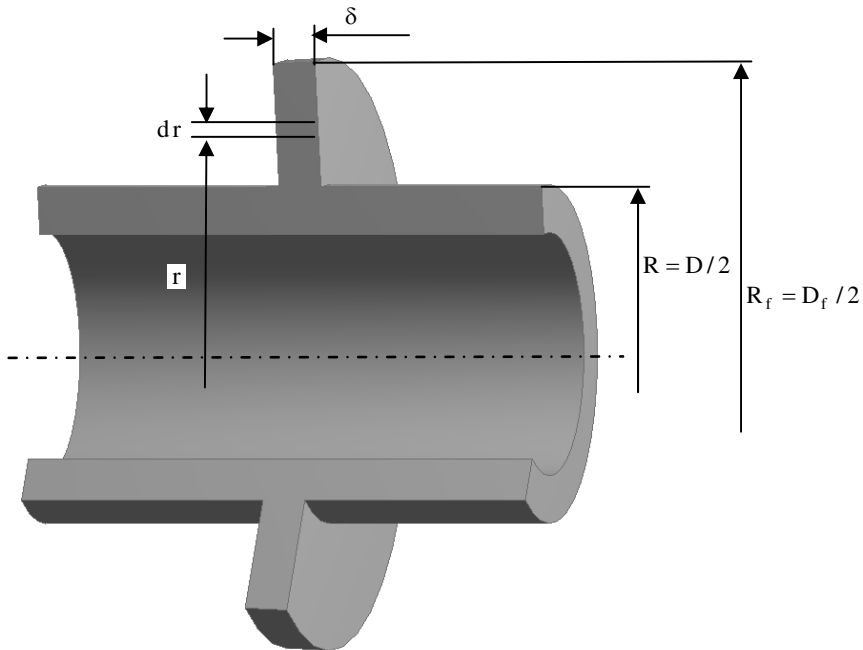
Fig. 3. Circular fin of uniform thickness.
