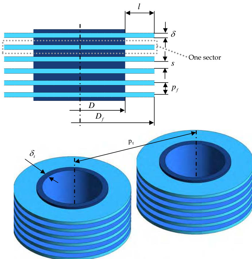
Fig. 6. Fin-tube geometry.
