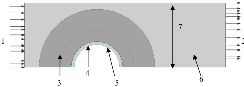
Fig. 5. Model used for CFD simulation.
