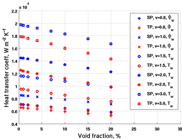
Fig. 15. Inside heat transfer coefficients for air-water flow.
