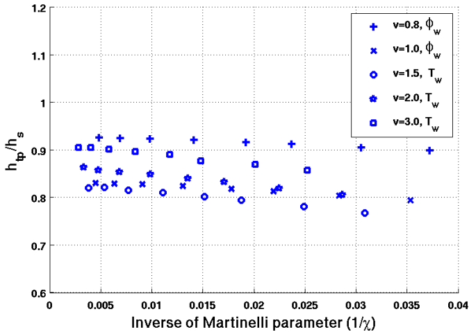
Fig. 16. Ratio h_{tp}/h_s as a function of \chi .
