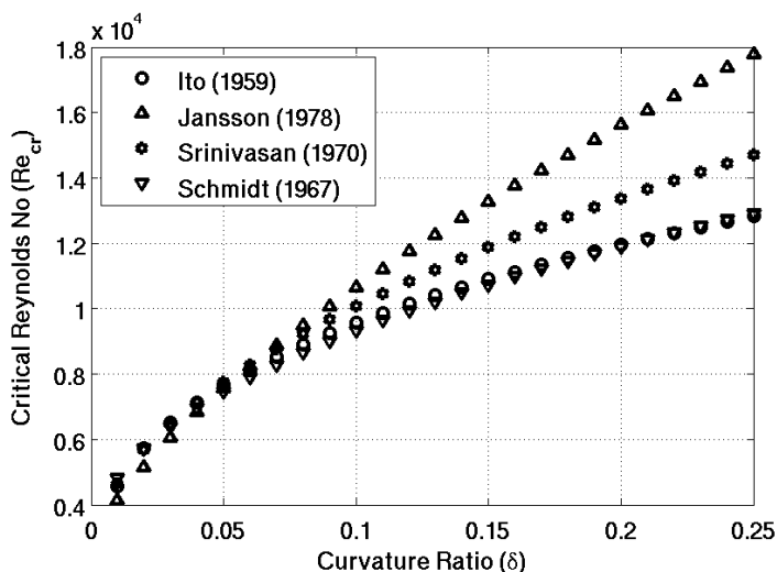
Fig. 2. Critical Reynolds number predicted by various correlations.
