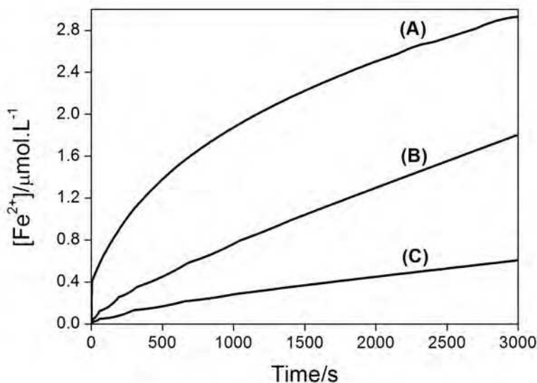
Fig. 6. The accumulation of ferrous ion during irradiation (350 nm) of 1.0 mM \text{Fe(III)} at: (A) pH 1.0 in the presence of 0.75\text{ mol L}^{-1} chloride ion; (B) at pH 3 in the absence of chloride ion; and (C) at pH 3 in the presence of 1.8\text{ mmol L}^{-1} sulfate ions.
