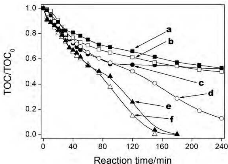
Fig. 3. Degradation of 12 mM phenol in the presence of 200 mM \text{H}_2\text{O}_2 and 0.5 mM \text{Fe}^{2+} . Fenton oxidation at \text{pH}_{\text{initial}} 3.0 in the presence (curve a, ■) and absence (curve b, □) of 0.5 M NaCl. Photo-Fenton degradation (400 W medium pressure Hg vapor lamp – incident photon intensities were 1.2 \times 10^{-4} Ein/s) at \text{pH}_{\text{initial}} 3.0 with no pH control in the absence (curve e, ▲) or presence (curve c, ●) of 0.5 M NaCl; or with pH 3.0 maintained throughout the reaction in the absence (curve f, △) or presence of 0.5 M NaCl (curve d, ○). For details, see (Machulek et al., 2007).
