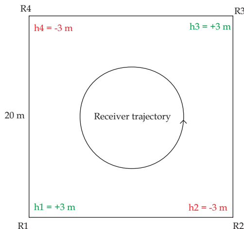
Fig. 25. Considered trajectory and repeater distribution
