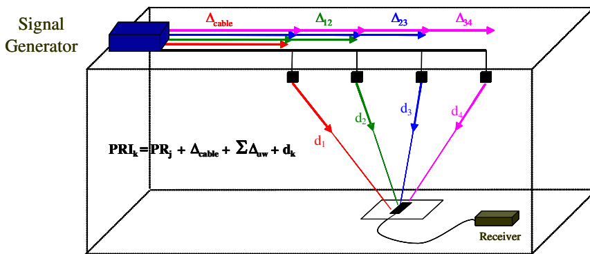
Fig. 23. The repealite system
