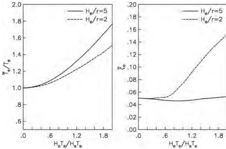
Fig. 7. Effect of SSI on the fundamental period and damping ratio of high- and low-rise structures on flexible foundation.
