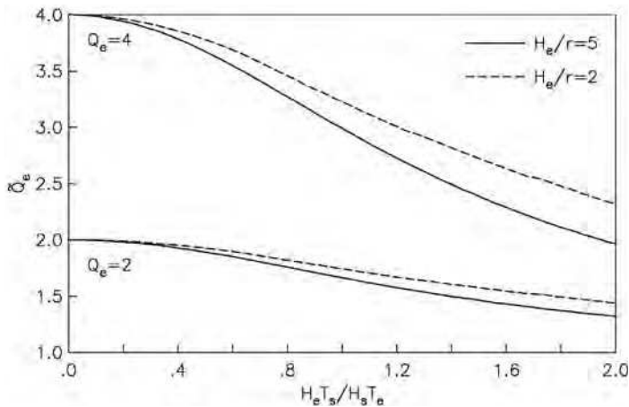
Fig. 8. Effect of SSI on the ductility factor of high- and low-rise structures on flexible foundation.
