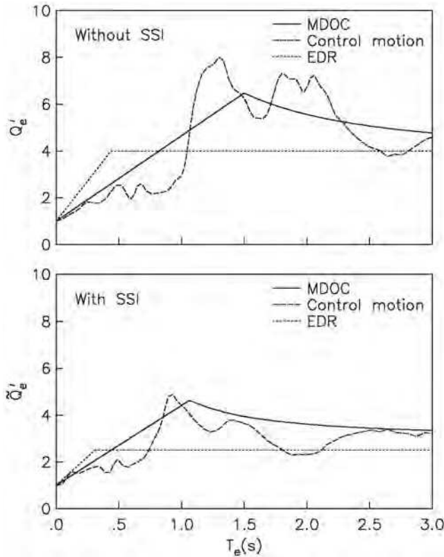
Fig. 11. Strength-reduction factors with and without SSI obtained from code provisions (MDOC and EDR) versus observations.
