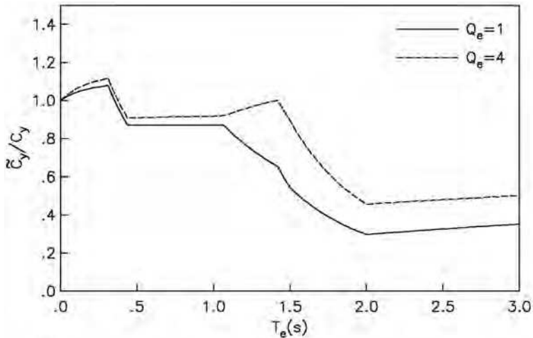
Fig. 13. Variation of the SSI factor for elastic and inelastic behavior.
