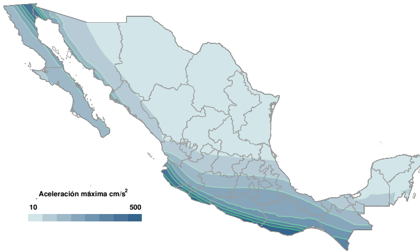
Fig. 2. Distribution of peak rock acceleration in Mexico for design of standard occupancy structures.
