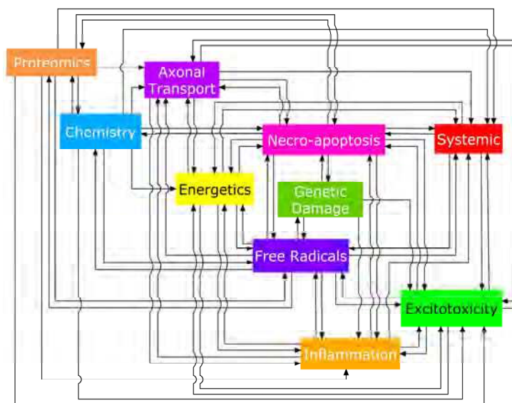
Fig. 1. Dynamic Meta-Analysis Feasibility Study Structure. Boxes represent the ten categories of outcome measures. Lines represent the 72 one-way interactions between categories of outcome measures. Systemics is shown in red as it represents the functional outcome metrics measured the in vivo G93A SOD1 mouse, and is used as the primary outcome for treatment evaluation (see Results). Categories are derived from the Phase II literature reviews. The outcome measures and their interactions are derived from the primary studies obtained from the Phase I literature search.
