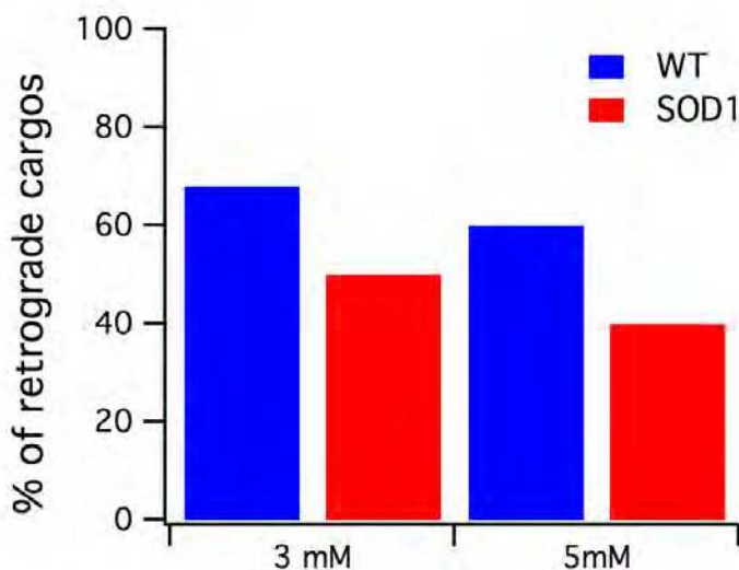
Fig. 3. Example data from a prototypical primary study.
