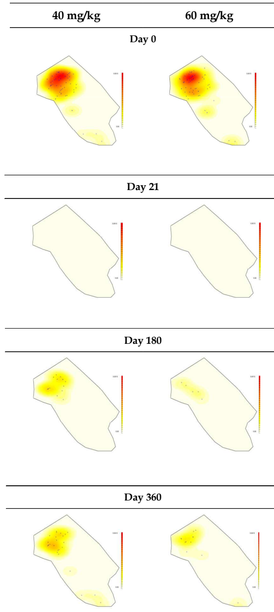
Fig. 1. Kernel intensity estimates of egg-positive subjects at baseline (Day 0), 21 days, 180 days and 360 days after treatment with PZQ 40 mg/kg or PZQ 60 mg/kg. The vertical bars indicate the kernel intensity scale. The original data are from Galvão et al., 2010.
