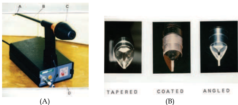
Fig. 10. (A) The IRK-151 infrared coagulator (a = tip; b = light-conducting quartz rod; c = reflector; d = timer). (B) Three kinds of artificial sapphire tips: (left) tapered, (middle) coated, and (right) angled. The coated tip has the same shape as the tapered tip, but the slanting surfaces are coated with nickel and tin dichloride. The angled tip has a 4-mm straight nose to prevent unnecessary ablation caused by direct contact of the slanting surface. When these sapphire tips are pressed into tissue, light energy is absorbed by the myocardium, which is then photocoagulated.
