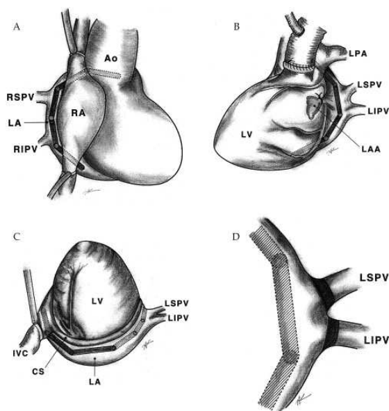
Fig. 7. Epicardial encircling cryoablation of the left atrium.
