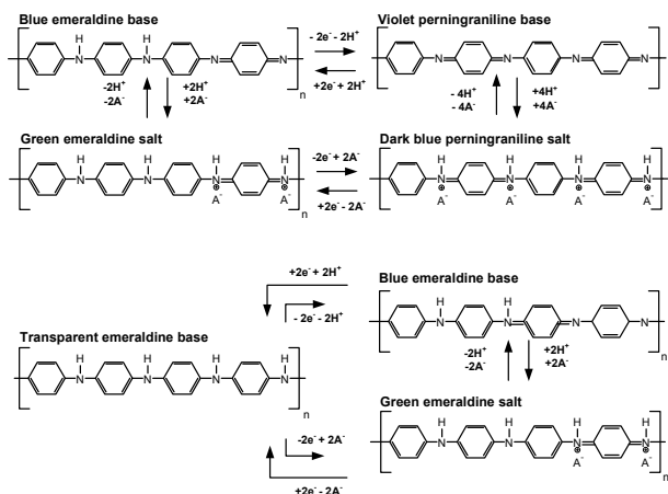
Fig. 1. Different forms of polyaniline
