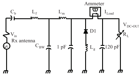
Fig. 11. Ultra low power DTV band rectenna circuit. SMS7630 Schottky diode by SKYWOKS offered the best performance.
