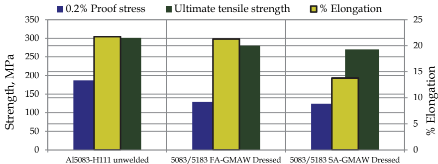
Fig. 23. Tensile Properties of 5083-H111/ER5183 welds.
