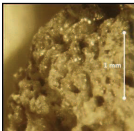
Fig. 1. Magnified view of a single expanded shale particle showing a highly porous exterior surface with range of pore sizes continuing into the interior of the particle
