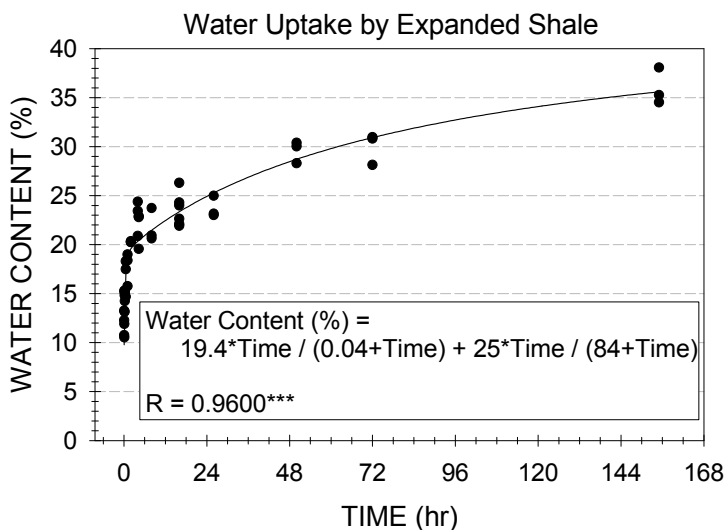
Fig. 2. Rate of water diffusion into expanded shale (EXSH) from a saturated porous medium. Data was fitted to a double rectangular hyperbolic function to create a predictive uptake equation. *** Significant at the 0.001 level of probability
