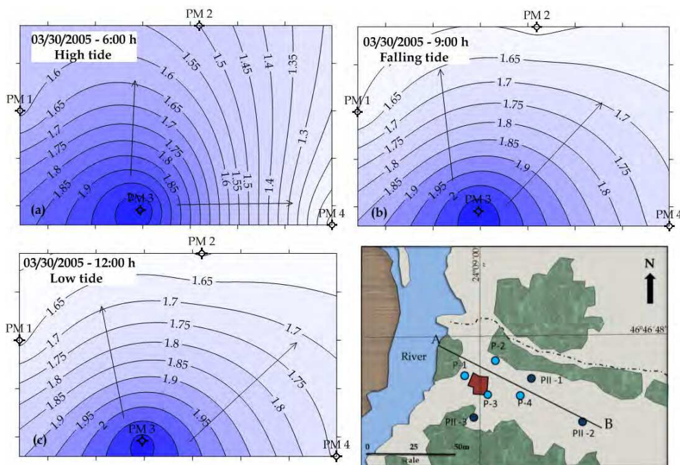
Fig. 9. Potentiometric surface maps representing groundwater flows in the following fluctuations: (a) high tide; (b) falling tide and (c) low tide - Shallow Aquifer (03/30/2005).
