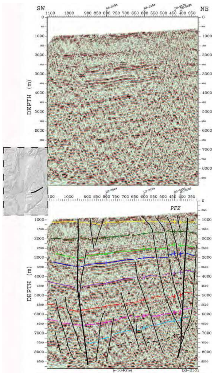
Fig. 4. DS-3101 depth section Datum +1,150m.; PFZ – Pezura Fault Zone. The Near Top Basement Horizon (H9) is assumed to lay ~1,000m below the Saramuj Fm (H8). Note the rising of the basement and the Saramuj Formation towards the PFZ on the eastern part of the profile. The western dip of the entire sedimentary column is clearly observable.
