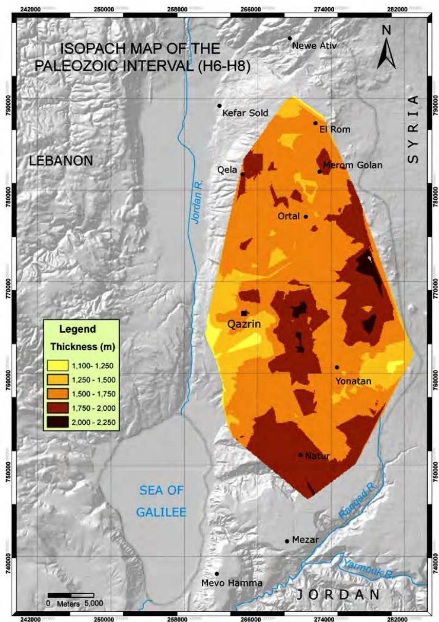
Fig. 10. Isopach map of the Paleozoic succession. The map represents the seismic interval calculated between H6 and H8.
