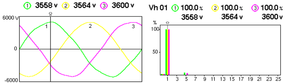
Fig. 7. Waveforms and harmonic spectra of the voltages in the intermediate state (MV Line)
