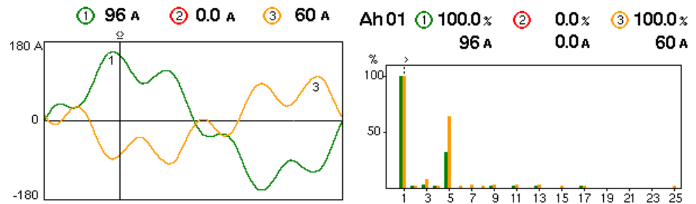
Fig. 9. Waveforms and harmonic spectra of the currents in the intermediate state (MV Line)
