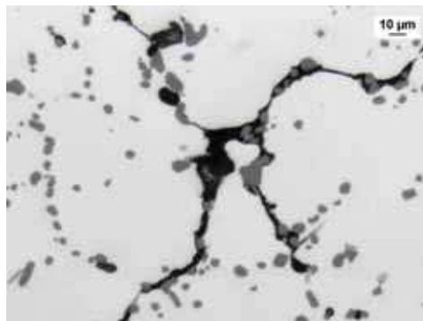
Fig. 13. Interdendritic and grain boundary incipient melting
