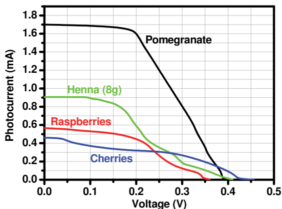
Fig. 14. Photocurrent vs. voltage curves obtained for nanostructured TiO_2 photoelectrodes sensitized with some extracted natural dyes (Jasim, submitted for publications).
