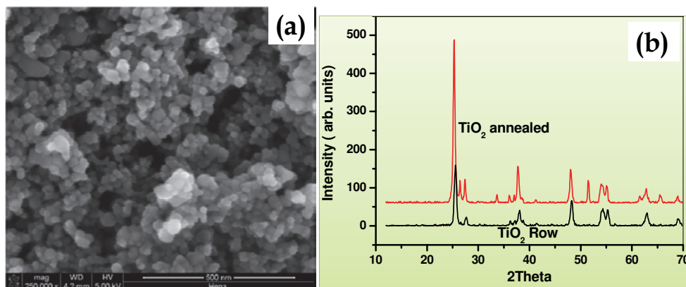
Fig. 5. (a) Scanning electron microscope (SEM) images and (b) XRD for TiO 2 photoelectrode before and after being annealed.
