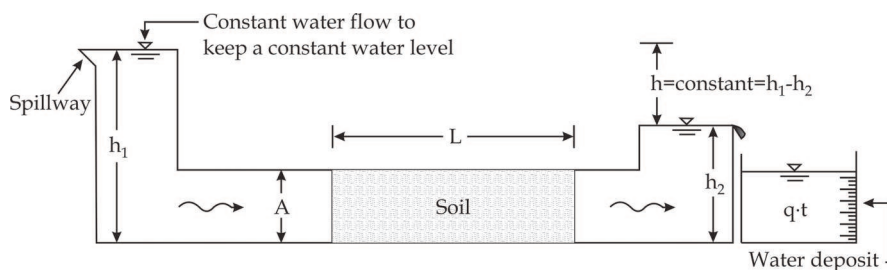
Fig. 5. Constant water head permeameter
