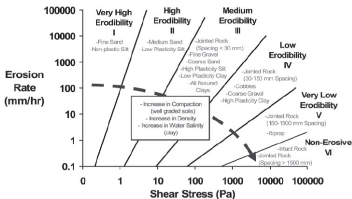
Fig. 4. Proposed erosion categories for soils and rocks based on shear stress (Briaud, 2008)
