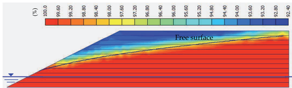
Fig. 14. Variation of degree of saturation for t = 4 d (345200 s) (Auvinet & Lopez-Acosta, 2010)
