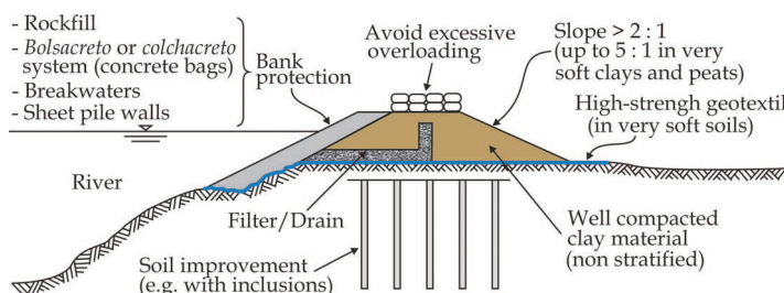
Fig. 10. Recommendations to protect levees on river banks (Auvinet et al., 2008)
