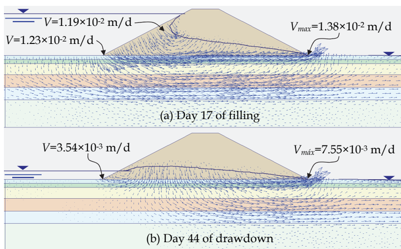
Fig. 22. Velocity vectors (magnitude) for two different time intervals during rapid filling and drawdown (exaggerated scale) (Lopez-Acosta et al., 2010)
