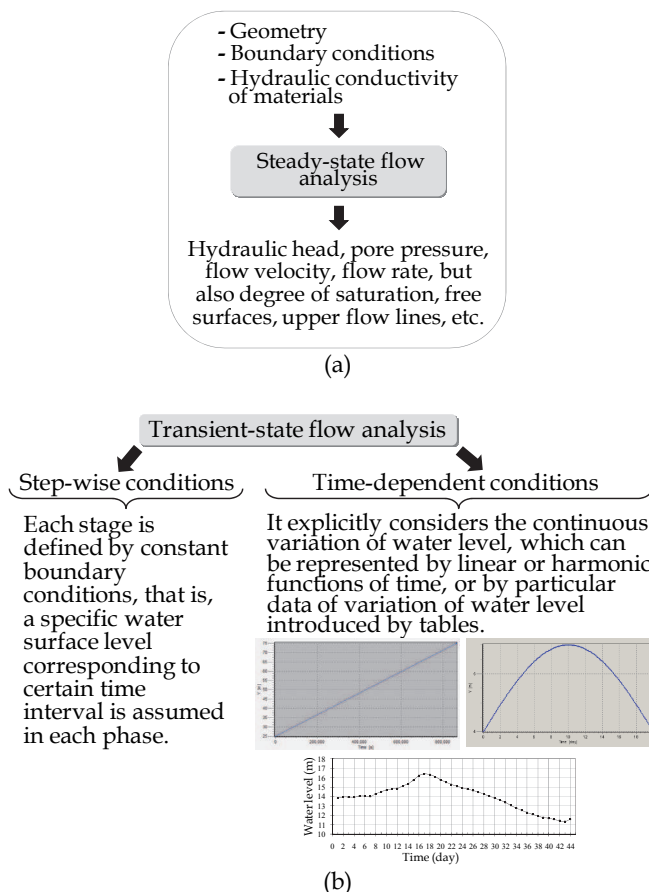
Fig. 8. Types of flow analyses performed with Plaxflow algorithm (Lopez-Acosta & Auvinet, 2010)
