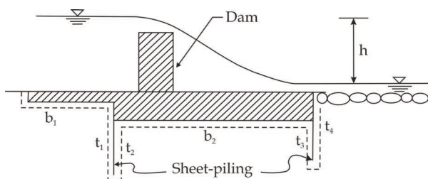
Fig. 1. Dam example given by Blight (1910) to define the percolation factor C_B (Casagrande, 1968)
