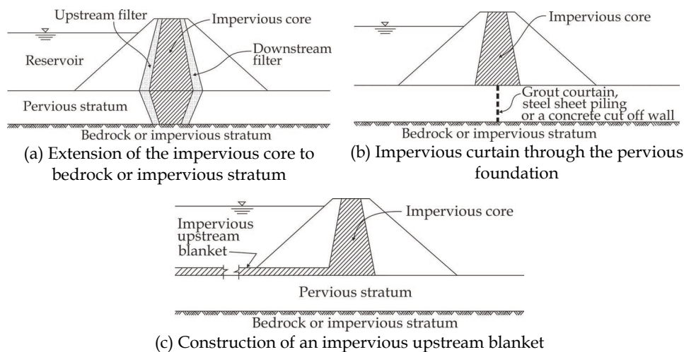
Fig. 9. Measures for preventing soil erosion or piping through a pervious foundation of an earth structure
