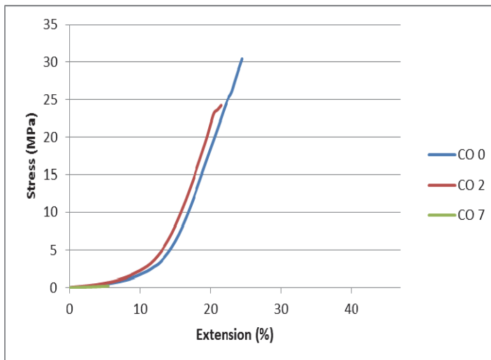
Fig. 13. Stress-elongation curves for cotton woven fabrics.
