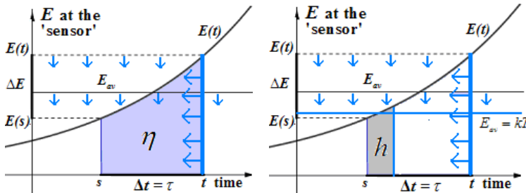
Fig. 3. E_0 = \frac{\Delta E}{\frac{\Delta E}{E_{av}} - 1} = \frac{\eta\nu}{e^{\eta\nu/\kappa\mathcal{T}_\eta} - 1}, \Delta E = \eta\nu, E_{av} = \kappa\mathcal{T}_\eta, \mathcal{T}_\eta = \left(\frac{1}{\kappa}\right)\frac{\eta}{\tau}, E(t) = E_0 e^{\nu t}
