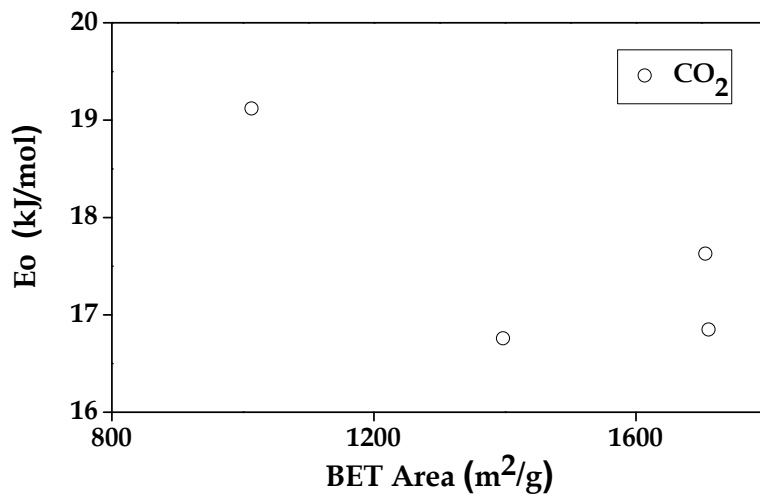
Fig. 25. Relationship between the characteristic energy and BET area of the series. a,b) COD. c,d) CUD.
