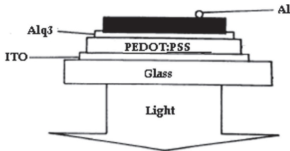
Fig. 1. Structure of Organic Light Emitting Diode.
