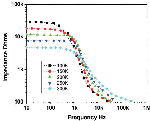
Fig. 14b. Impedance spectra of ITO/PEDOT:PSS/MEH:PPV/LiF/Al.
