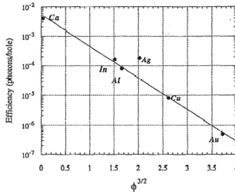
Fig. 7. Device Efficiency v (Barrier Height) 3/2 [I.D.Parker,1994].
