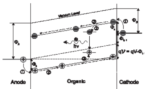
Fig. 3. Basic Steps of Electroluminescence with Energy Band[4].
