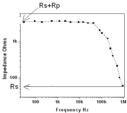
Fig. 12. Deducing equivalent circuit from impedance plots.
