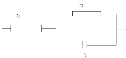
Fig. 12. Deducing equivalent circuit from impedance plots.
