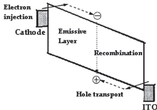
Fig. 2. Injection, Transport and Recombination in PLED[15].
