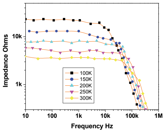
Fig. 14a. Impedance spectra of ITO/PEDOT:PSS/MEH:PPV/Al.
