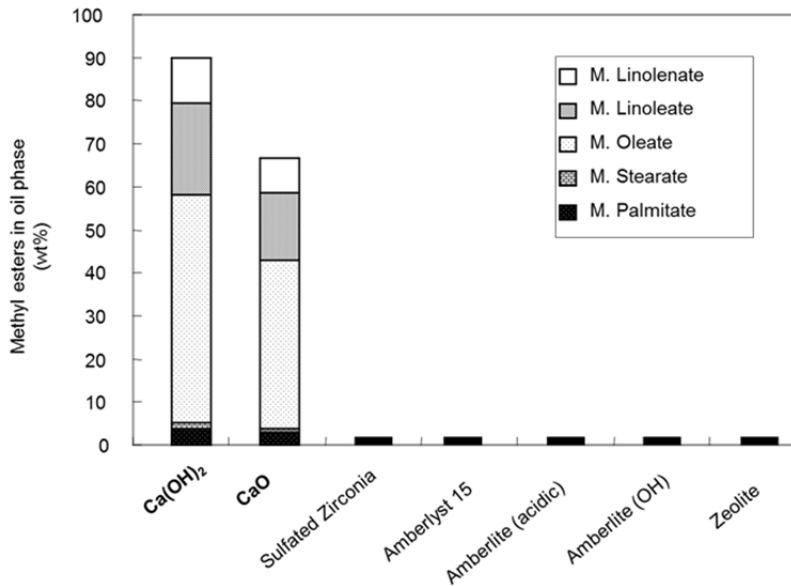
Fig. 5. Comparison of activities of various catalysts under microwave irradiation ( t = 1\text{min} , catalysts = 10g, MW = 700W)
