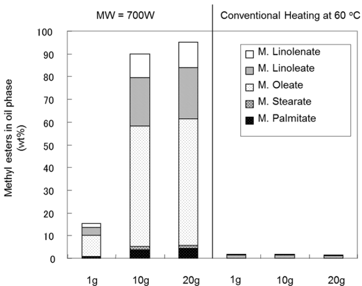
Fig. 6. Comparison of microwave and conventional heating (t = 1min, catalysts: Ca(OH) 2 , MW = 700W)
