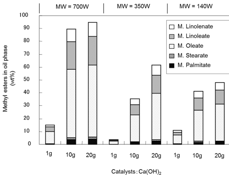
Fig. 7. Dependency of yield on microwave irradiation power at various amounts of Ca(OH) 2 catalysts (t=1min)
