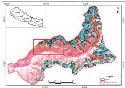
Fig. 9d. Glaciers in 2009
