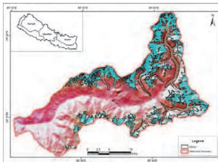
Fig. 9c. Glaciers in 2000
